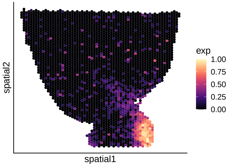
S100a5: simualte data 90% signal
