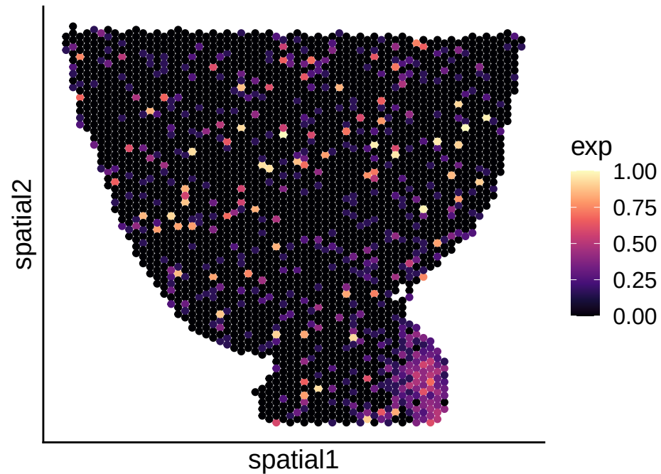
S100a5: simualte data 10% signal
