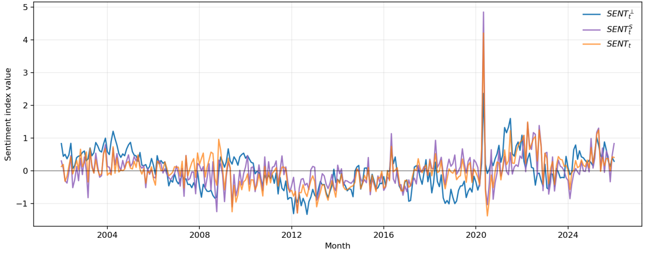
Figure 1: Raw and macro-orthogonalized Swedish dividend-premium sentiment indices
