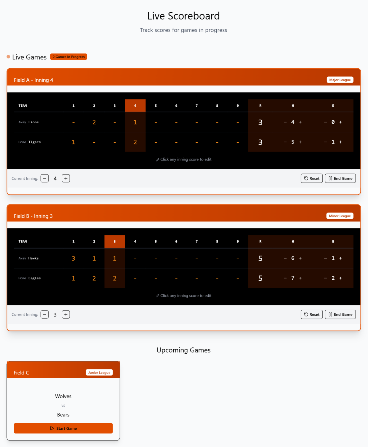
Figure 31: Live Score
