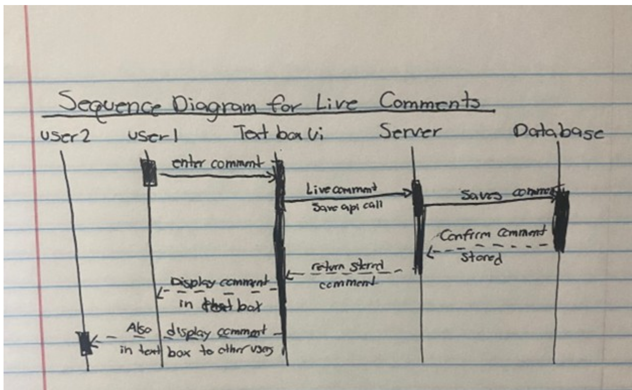
Figure 1: Sequence Diagram for Live Comments
