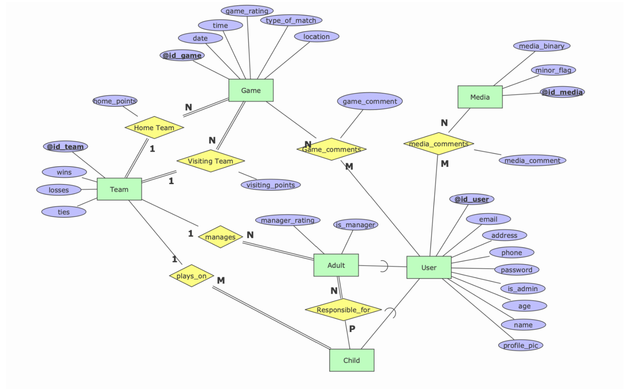
Figure 3: Our ERD
