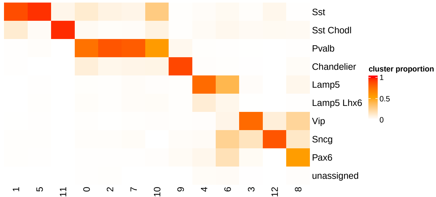
wang-rat cluster predictions with homologous mouse markers
