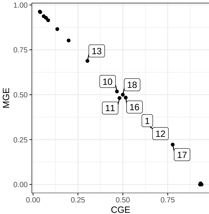
Mouse CGE-MGE cluster proportions: W
