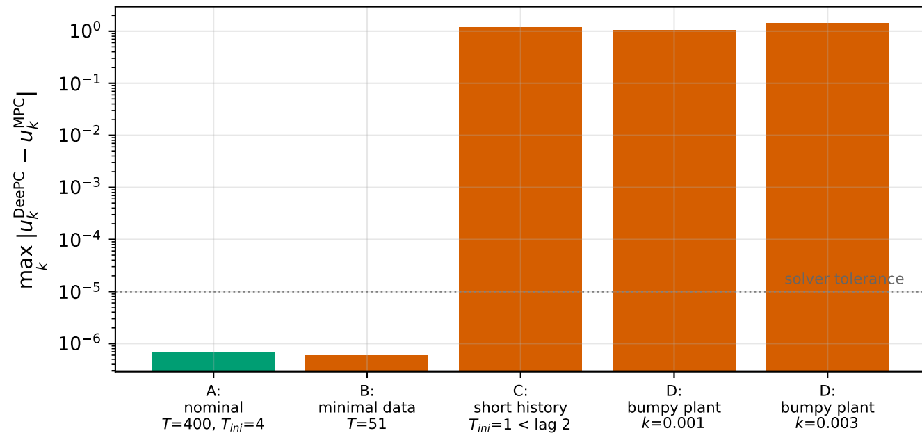
Input deviation from the exact-model MPC
