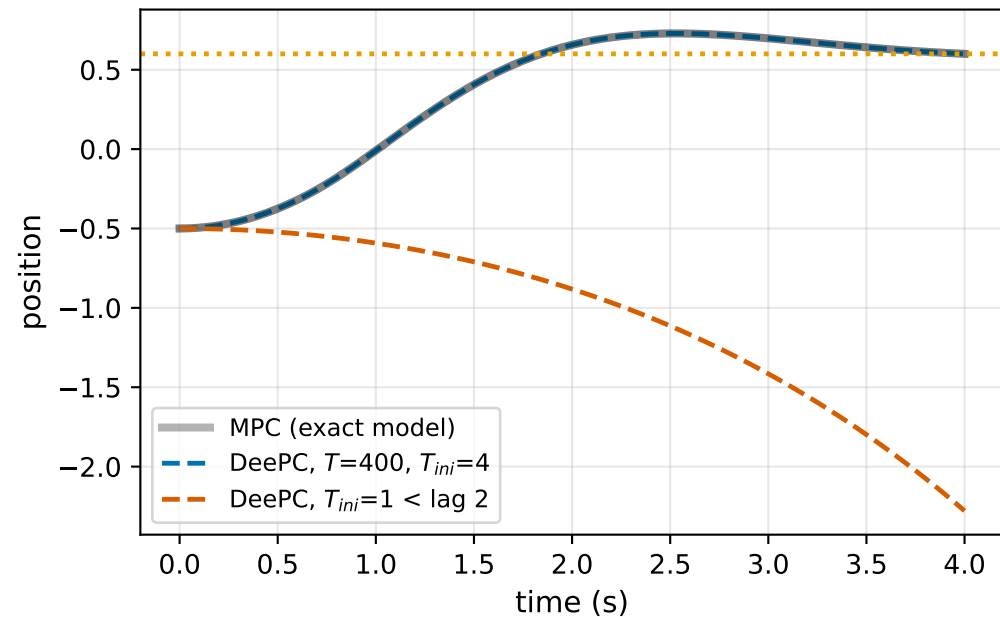
Closed loop: nominal vs. too short history
