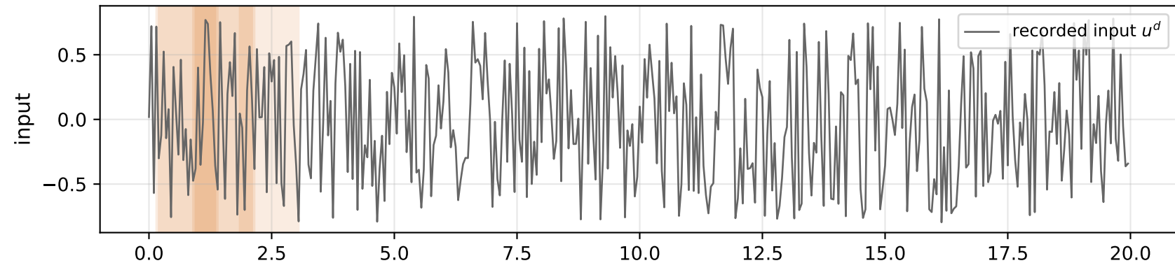
The five most heavily weighted windows of the experiment (shaded, length L \Delta t )
