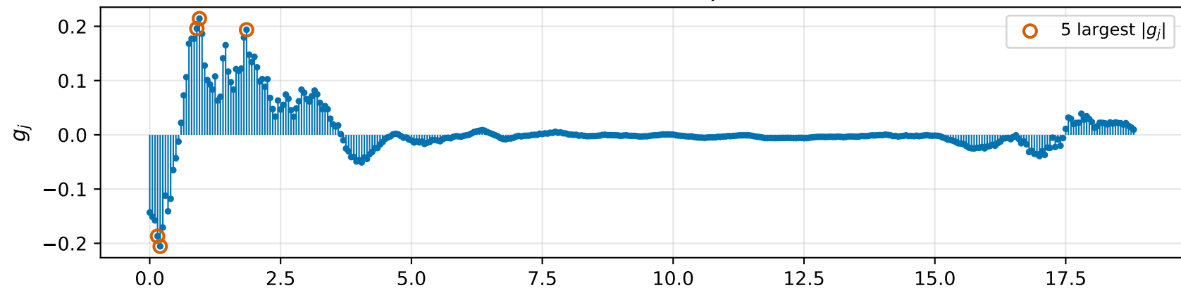
Behavioral coefficient g over the start time t_j of the data window it weights
