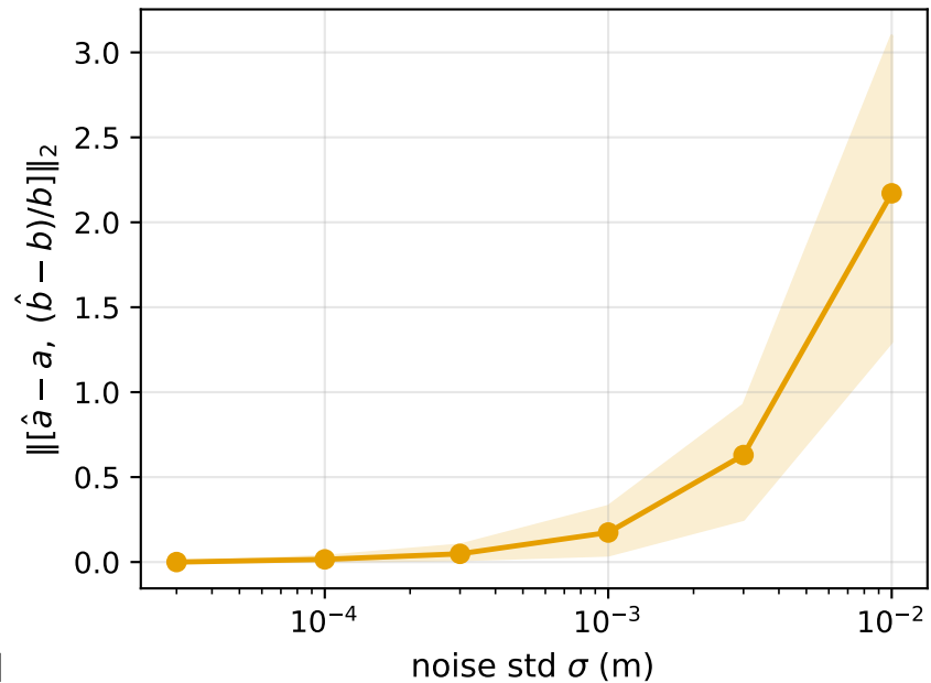
Least-squares model error (indirect route)
