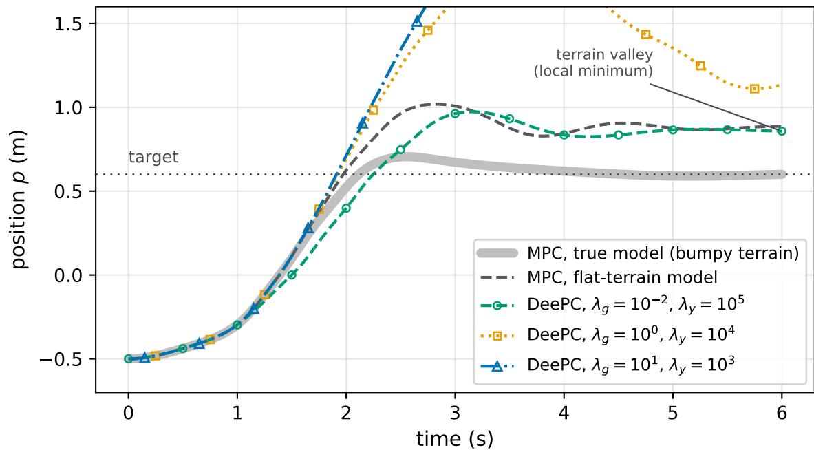
Closed-loop trajectories
