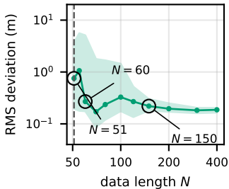
DeePC tracking performance
