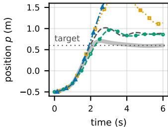
closed-loop trajectory
