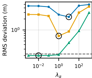
DeePC tracking performance
