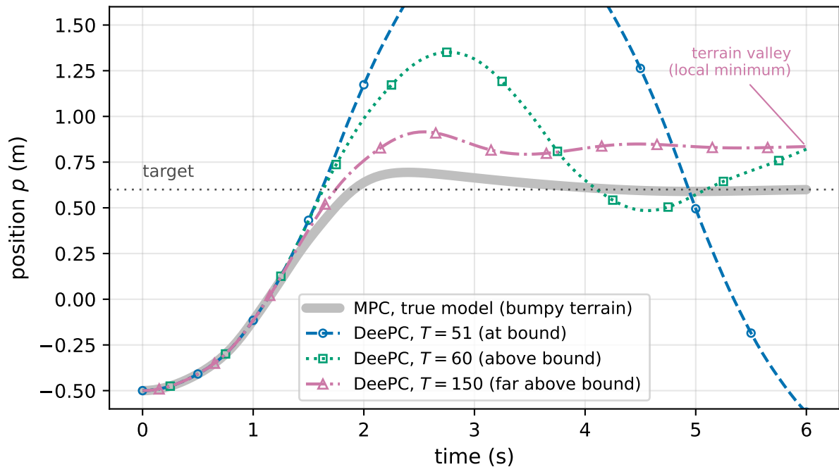
Closed-loop trajectories (one data record)
