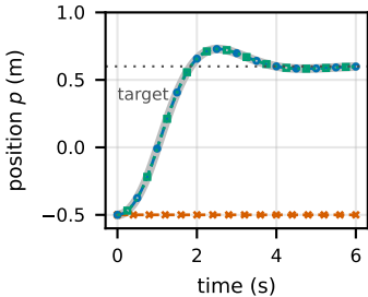
Closed-loop trajectory
