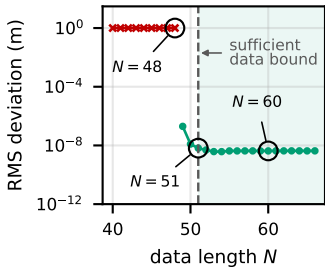
DeePC tracking error
