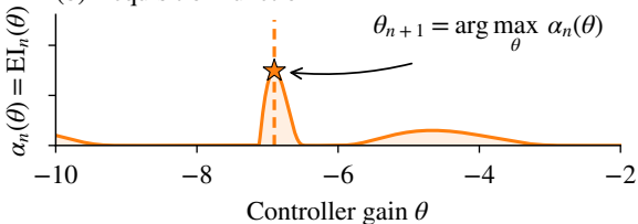
(b) Acquisition function
