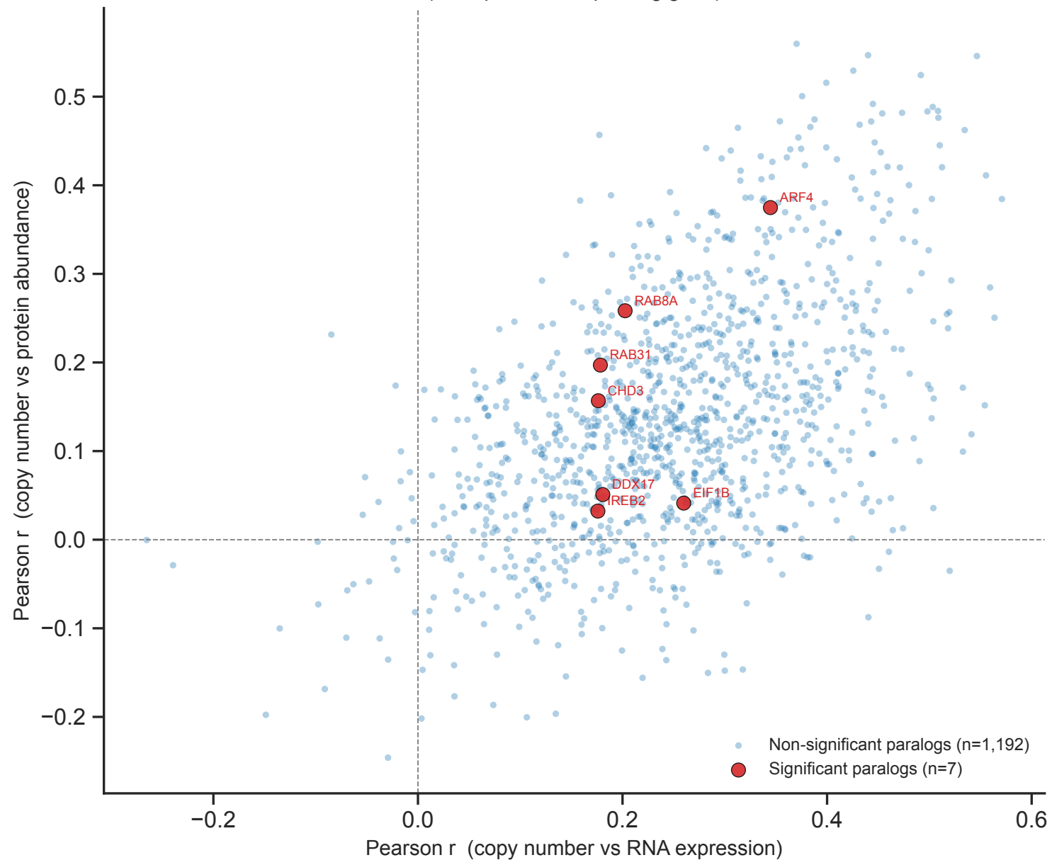
CN-expression coupling across CCLE cell lines (each point = one paralog gene)
