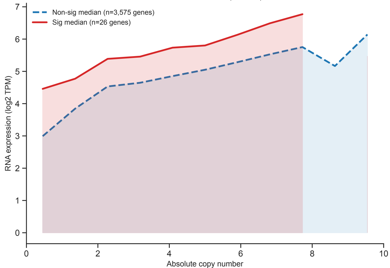
Copy number vs RNA expression (log2 TPM) across CCLE cell lines (CN \leq 10 )
