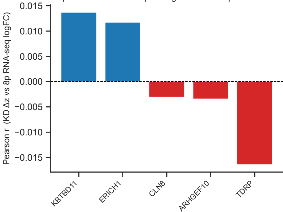
Transcriptional correlation of 8p KD signatures with 8p deletion RNA-seq
