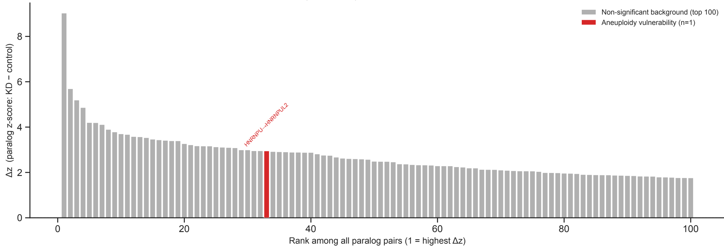
Top 100 paralog pairs by \Delta z — K562_essential Aneuploidy vulnerability pairs in red (total ranked: 1,610)
