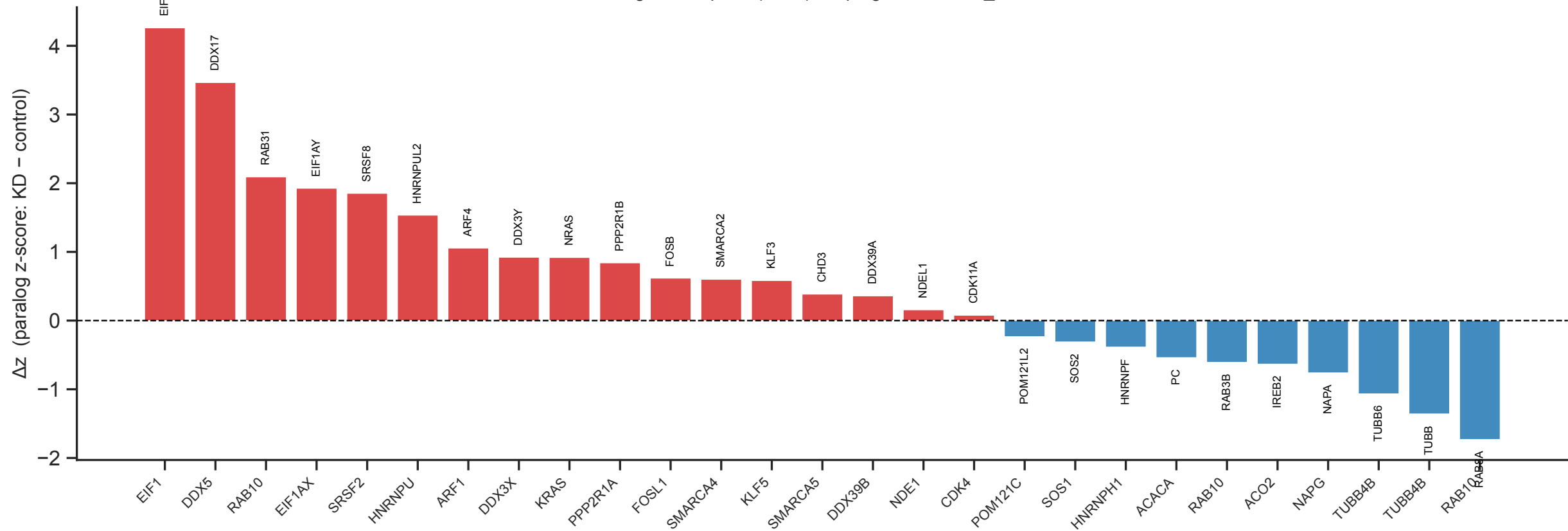
Paralog upregulation upon dep_gene CRISPRi knockdown Significant pairs (n=27), Replogle 2022 cd4t_rest
