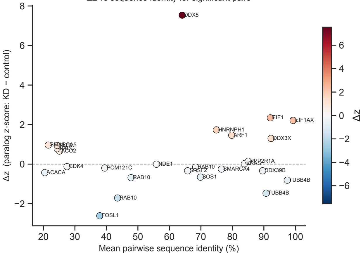
\Delta z vs sequence identity for significant pairs
