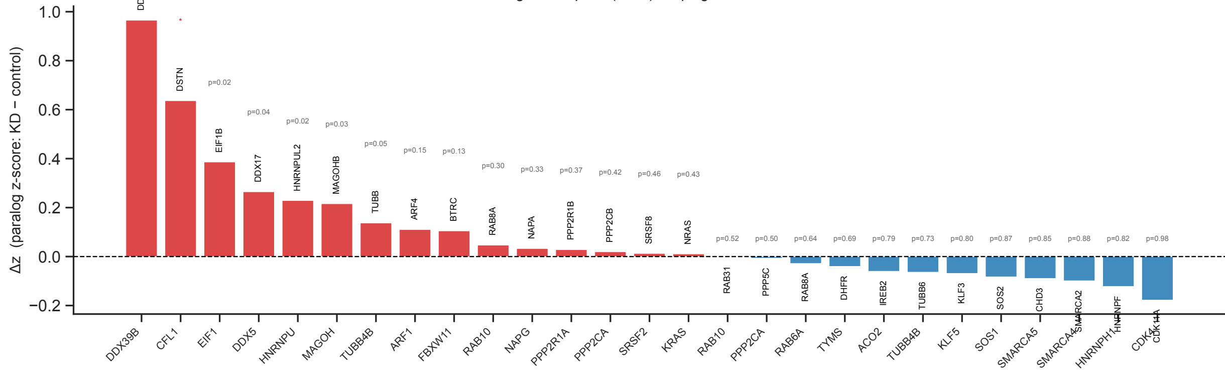
Paralog upregulation upon dep_gene CRISPRi knockdown Significant pairs (n=27), Replogle 2022 K562
