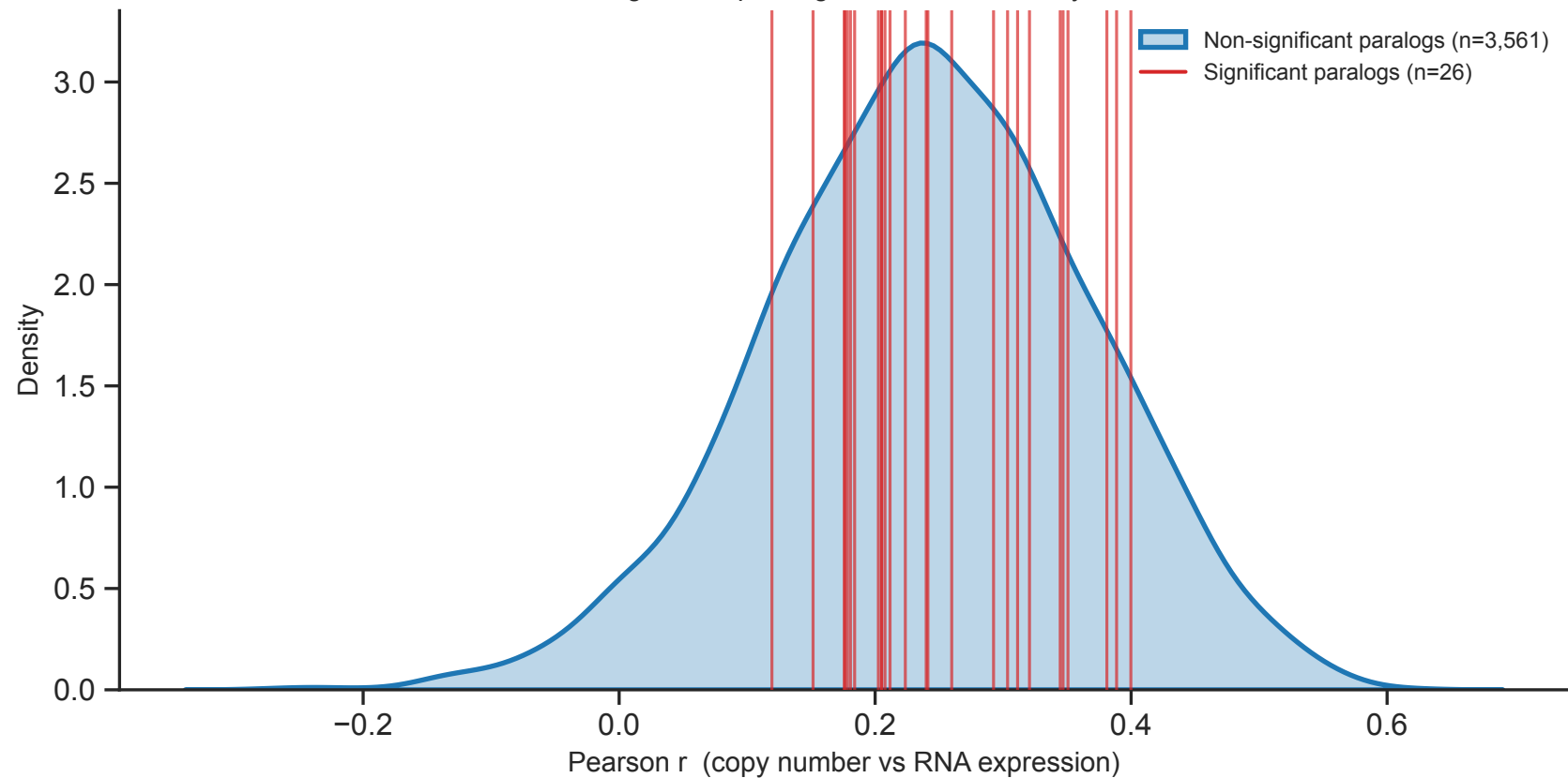
Distribution of CN-RNA coupling across paralog genes Significant paralogs marked individually
