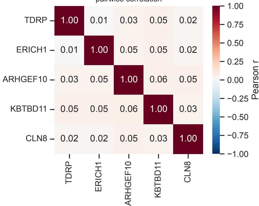
8p common-region gene KD signatures pairwise correlation
