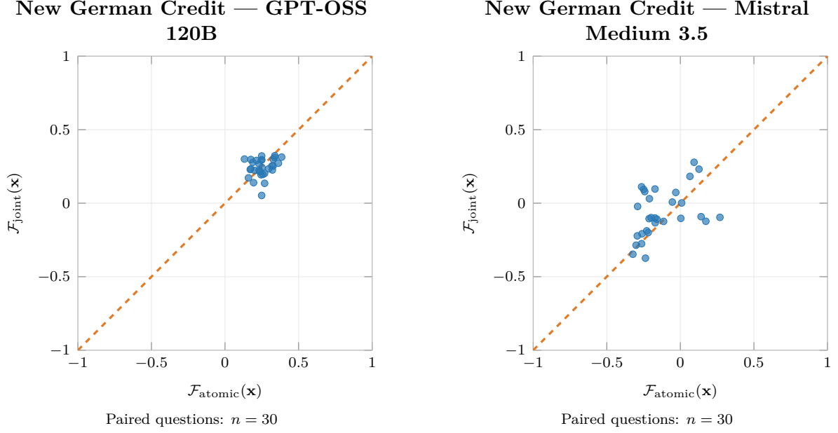
Figure 7.8: Question-level atomic and joint faithfulness for New German Credit (continued).
