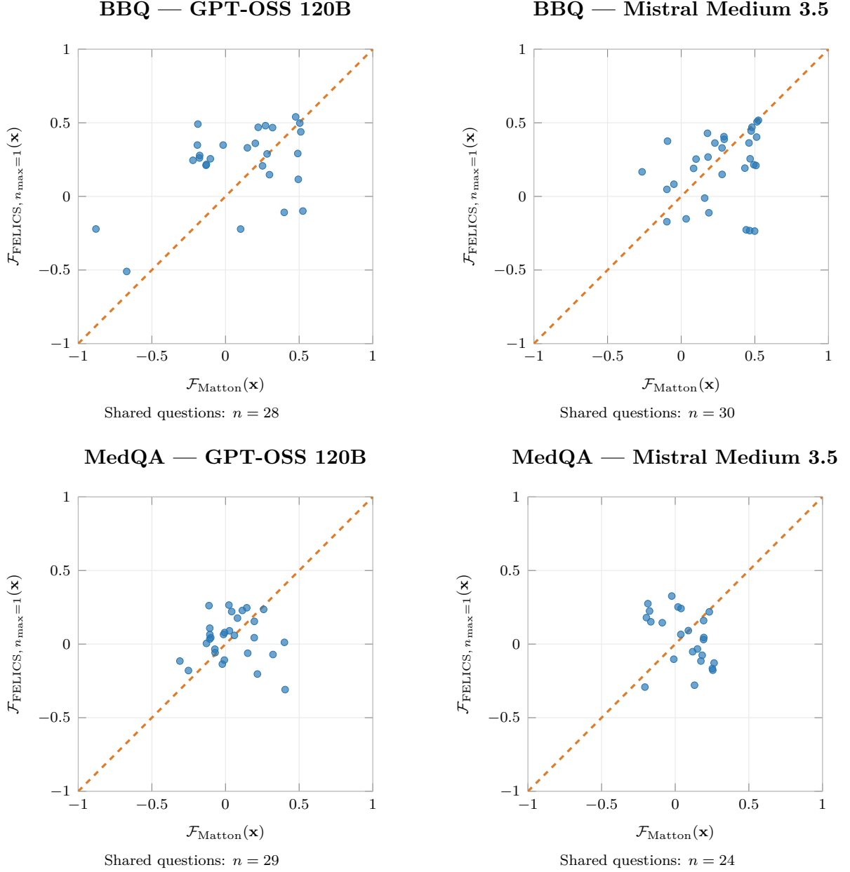
Figure 7.6: Question-level faithfulness produced by FELICS with n_{\max} = 1 and the original Matton implementation for the four natural-language comparisons.
