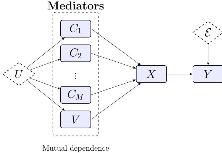
Figure 3.1: The data generating process for one single original dataset question and the model response, as assumed by Matton et al. [MNGK25].
