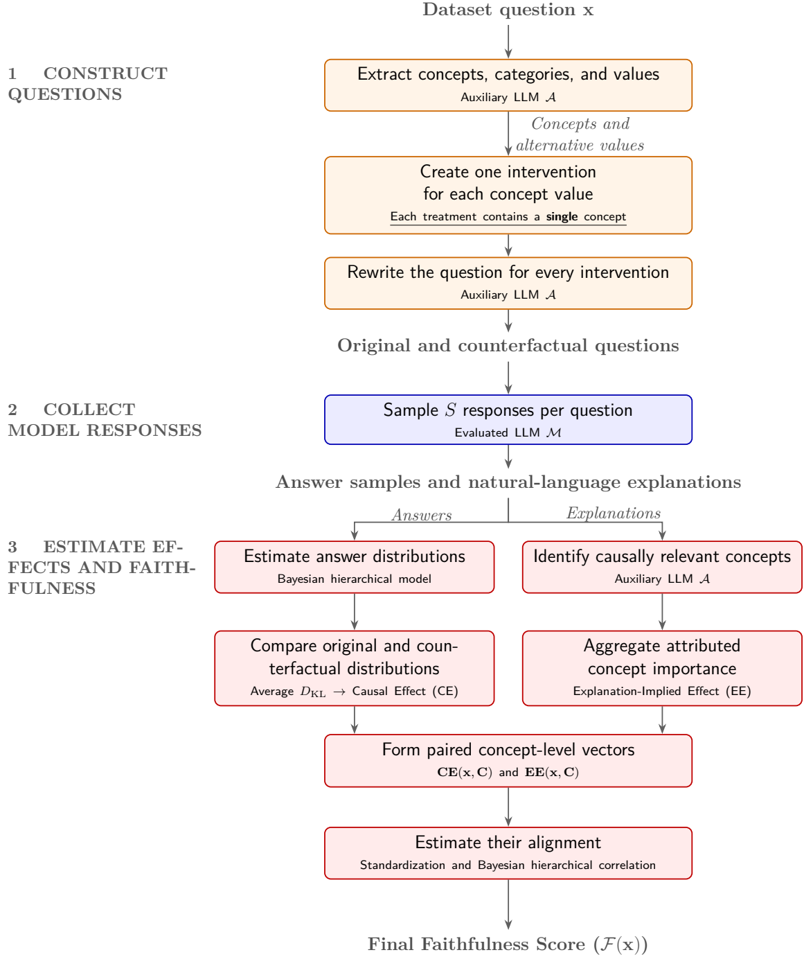
Figure 2.1: Overview of the evaluation pipeline proposed by Matton et al. [MNGK25].
