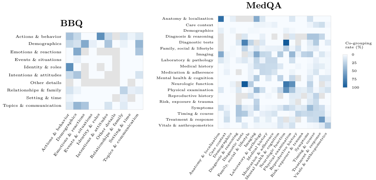
Figure 7.2: Co-grouping rates for the natural-language oracle on LLM-normalized Categories
