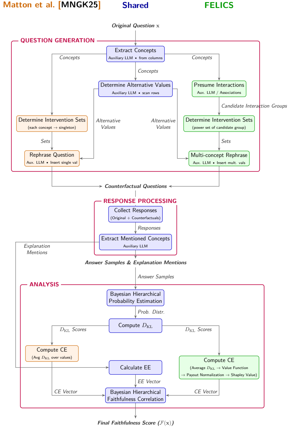
Figure 5.1: Comparison of the evaluation pipeline between Matton et al. [MNGK25] (left) and the proposed FELICS framework (right) with highlighted modifications.
