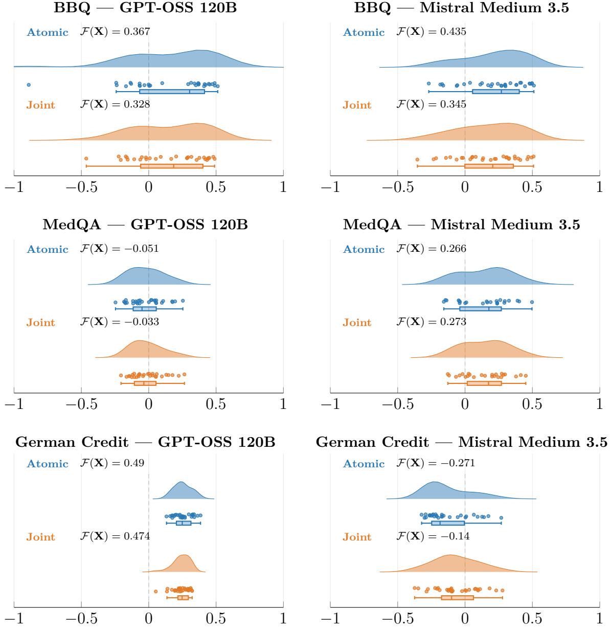
Figure 7.1: Distribution of question-level faithfulness based on atomic and interaction-aware causal effects from the same joint FELICS run on different dataset/model combinations.
