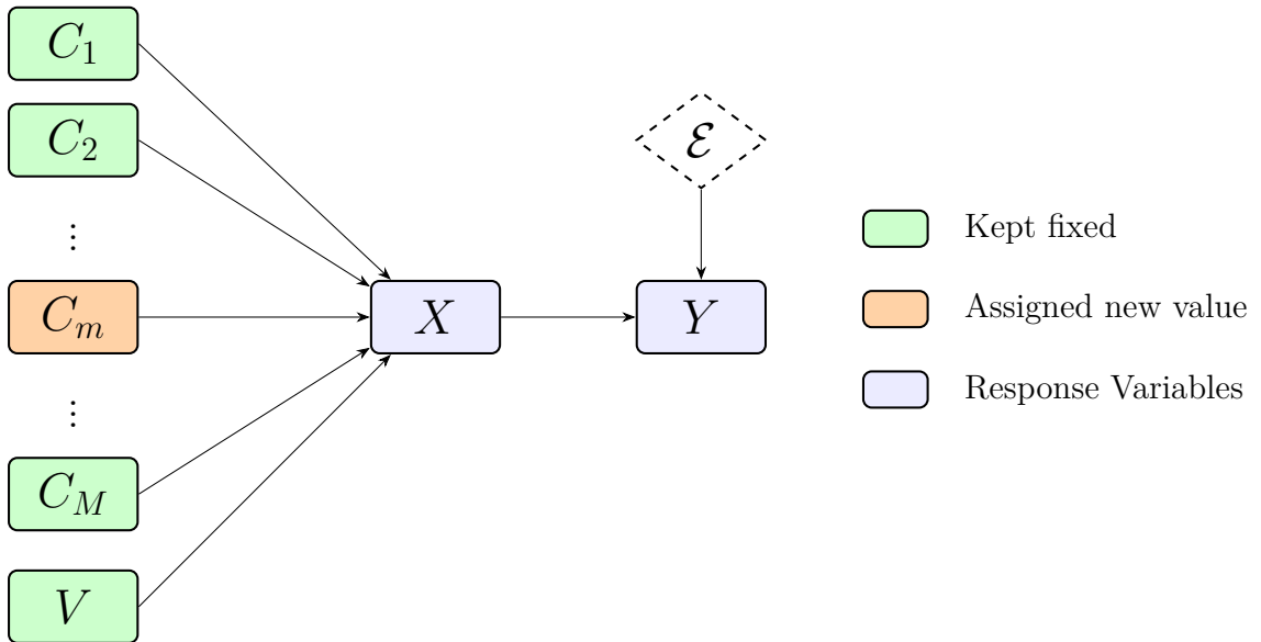
Figure 3.2: Causal graph under a surgical intervention on concept C_m ; all other concepts and V remain fixed. Adapted from [MNGK25a].
