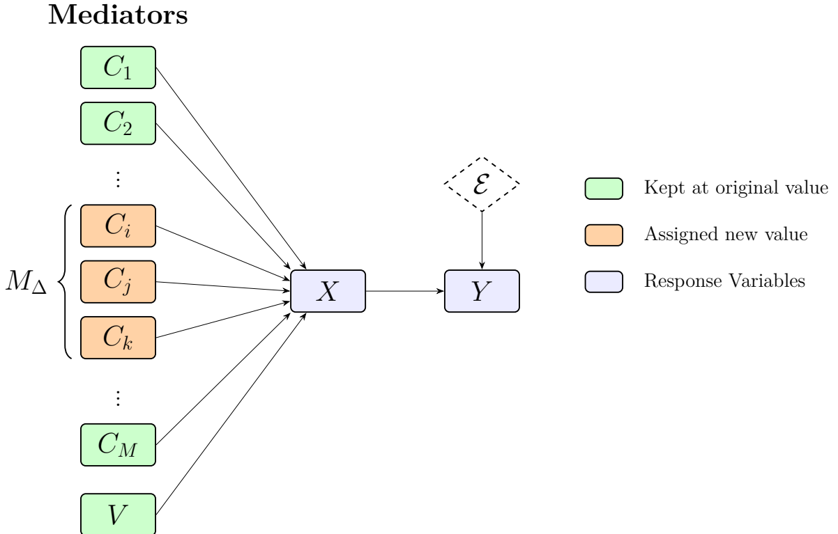
Figure 5.1: Causal graph under a joint intervention on the concepts C_i with i \in M_{\Delta} . All remaining concepts ( i \notin M_{\Delta} ) and the rest-of-question text V remain fixed.
