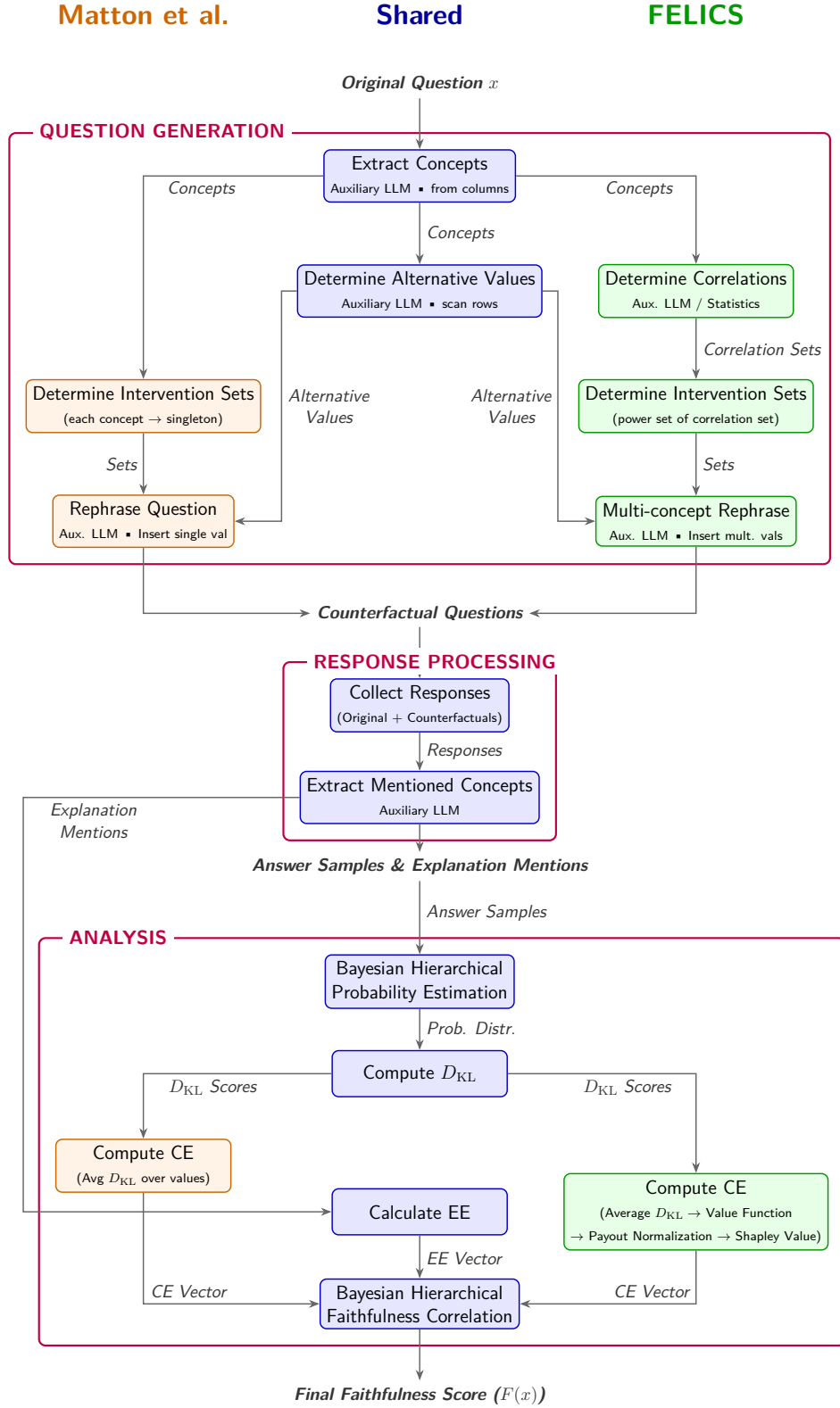
Figure 6.1: Comparison of the evaluation pipeline between Matton et al. [MNG24] (left) and the proposed FELICS framework (right), highlighting their shared foundations as well as the modifications to intervention generation and causal-effect estimation.
