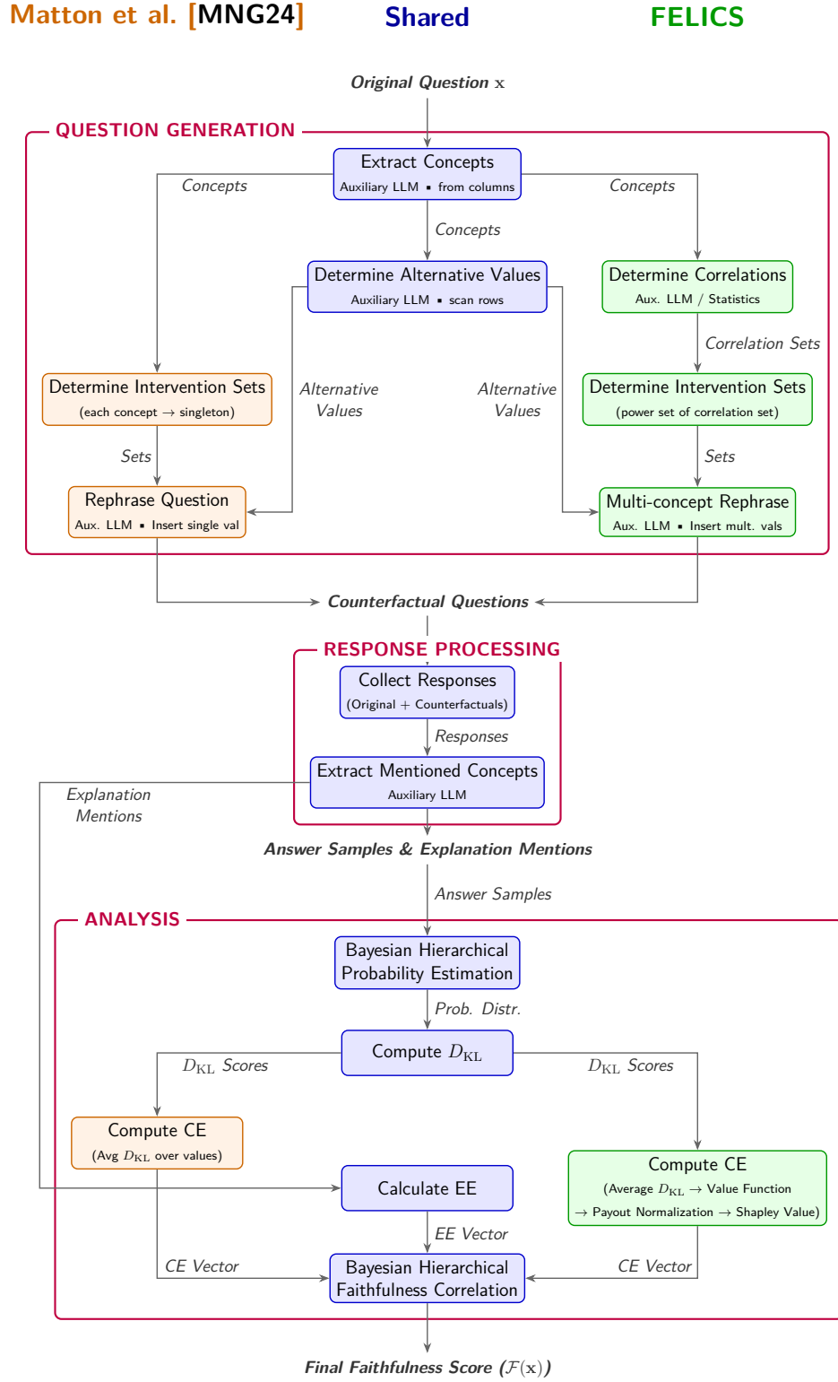
Figure 5.1: Comparison of the evaluation pipeline between Matton et al. [MNG24] (left) and the proposed FELICS framework (right) with highlighted modifications.
