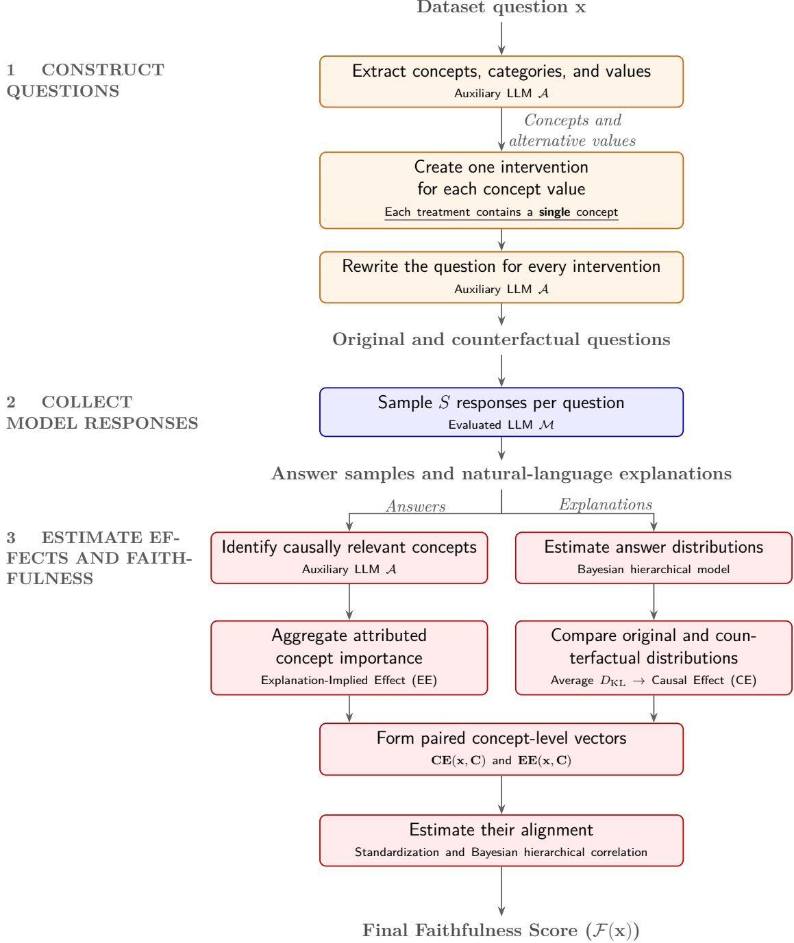
Figure 2.1: Overview of the evaluation pipeline proposed by Matton et al. [MNG24]. The flow summarizes the construction of counterfactual questions, collection of model responses, estimation of causal and explanation-implied effects, and aggregation into a final question-level faithfulness score.
