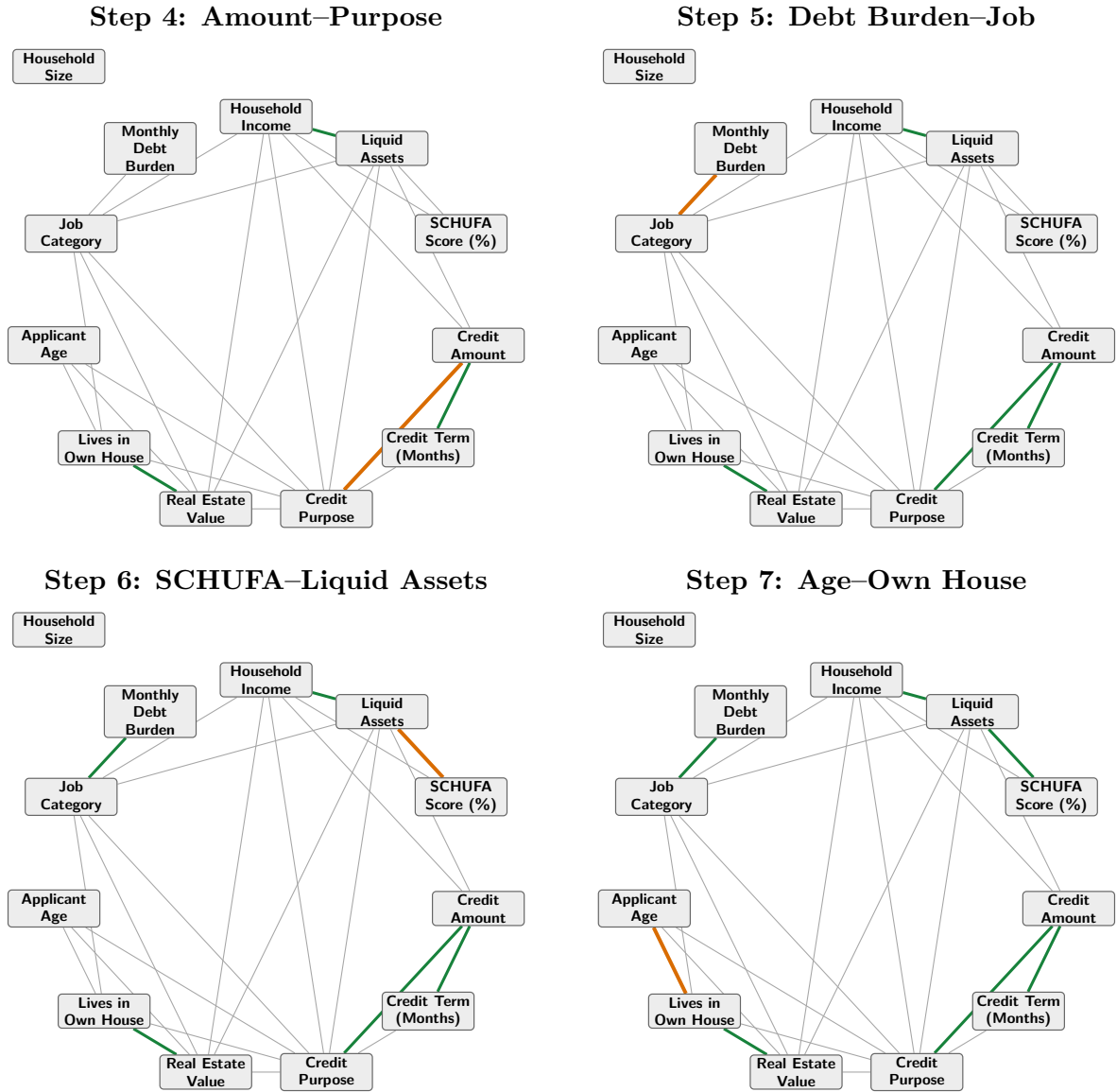
Figure C.2: The final four accepted merges of the New German Credit partitioning algorithm. The last panel is the completed maximum spanning forest.
