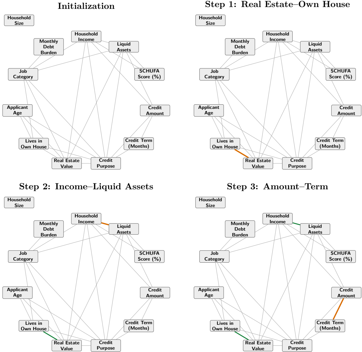
Figure C.1: Initialization and the first three accepted merges of the New German Credit partitioning algorithm.
