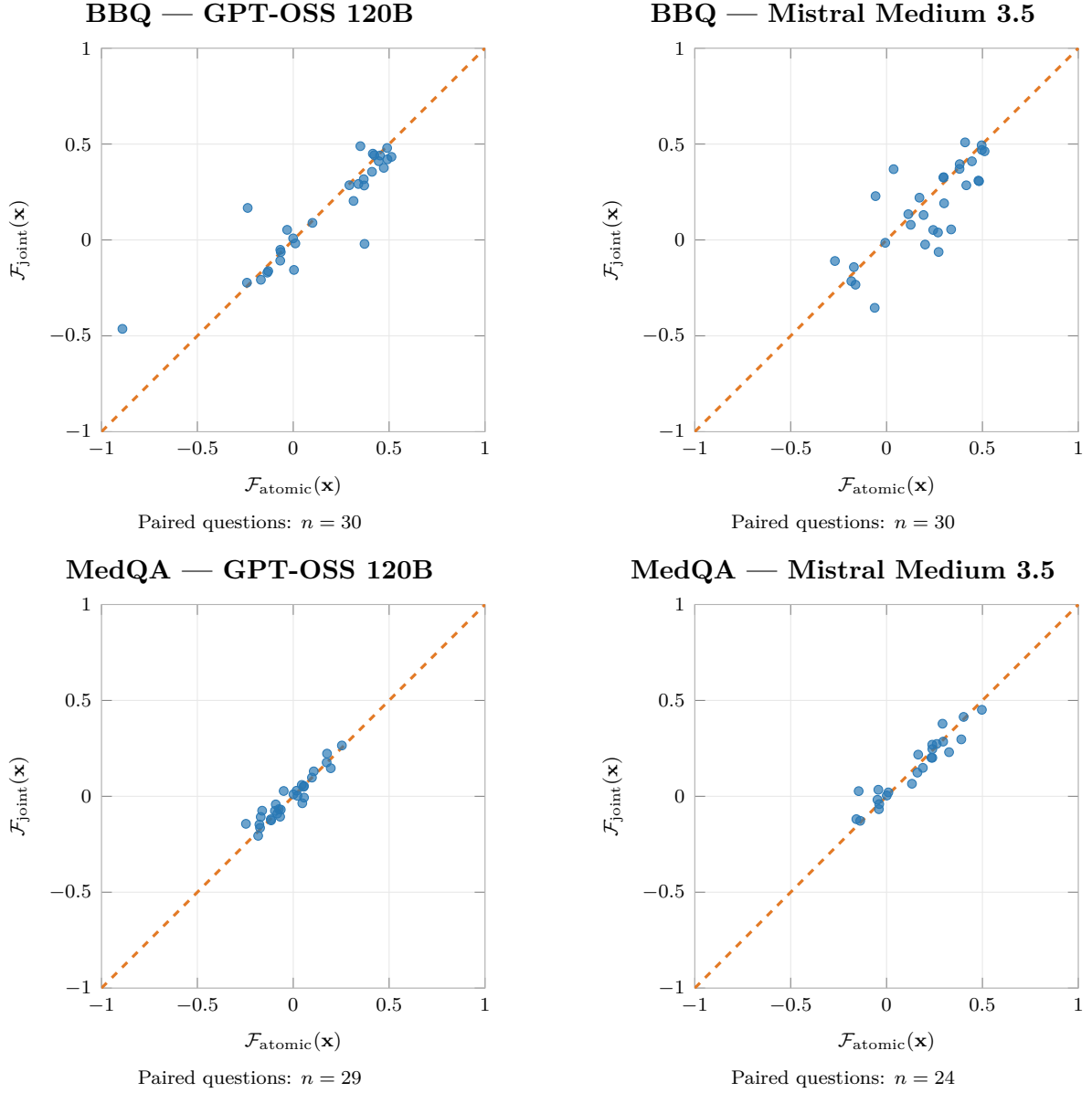
Figure 7.8: Question-level atomic and joint faithfulness for BBQ and MedQA.
