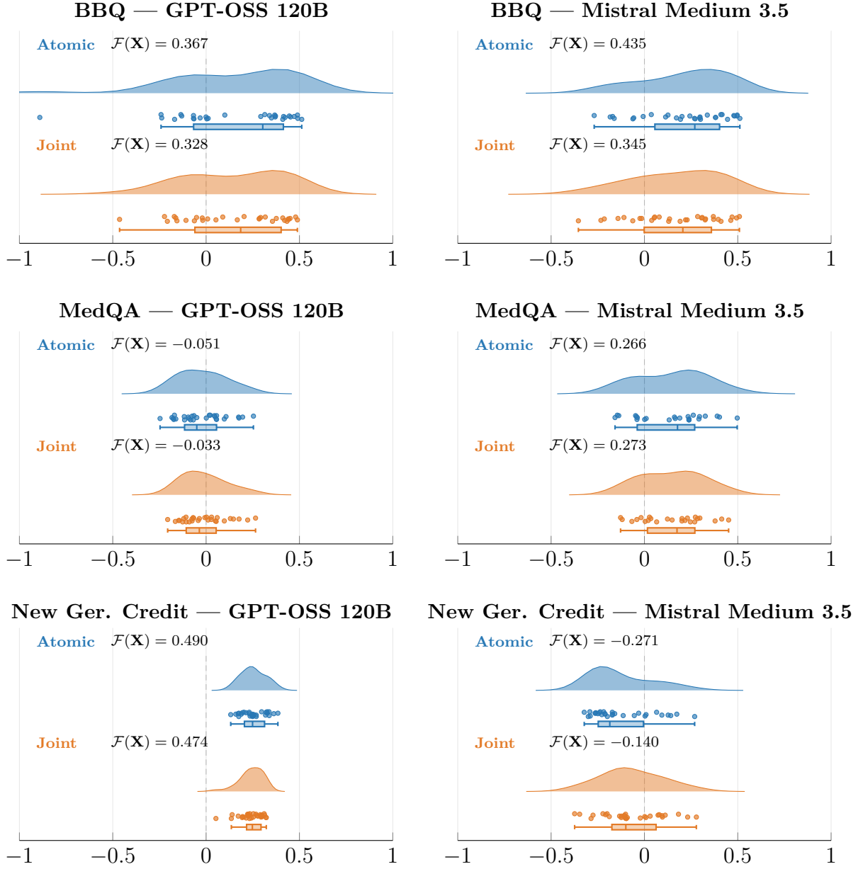
Figure 7.1: Distribution of question-level faithfulness based on atomic and interaction-aware causal effects from the same joint FELICS run on different dataset/model combinations.
