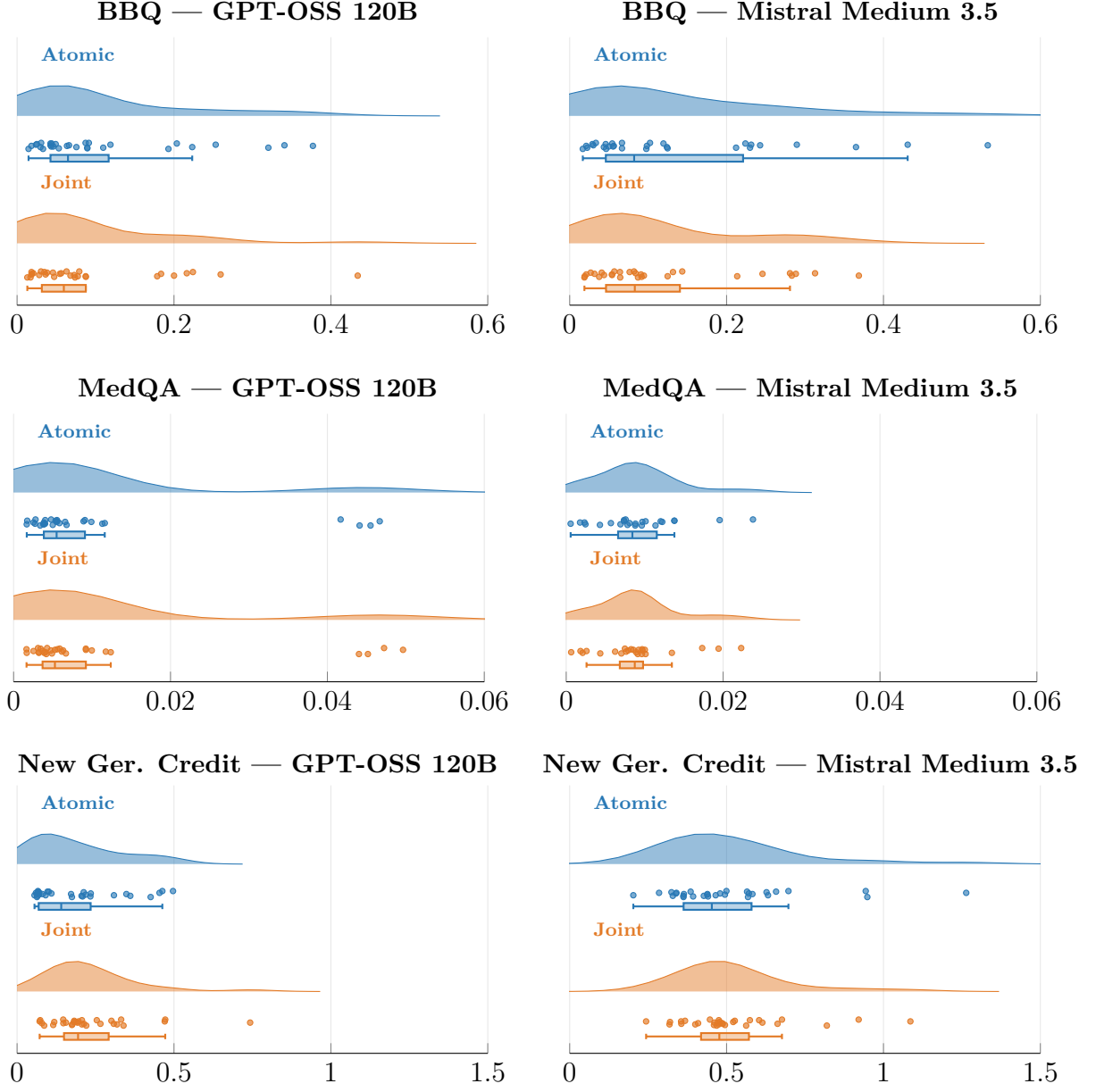
Figure D.1: Distribution of question-averaged causal effects obtained from the atomic and interaction-aware CE vectors of the same joint FELICS runs.
