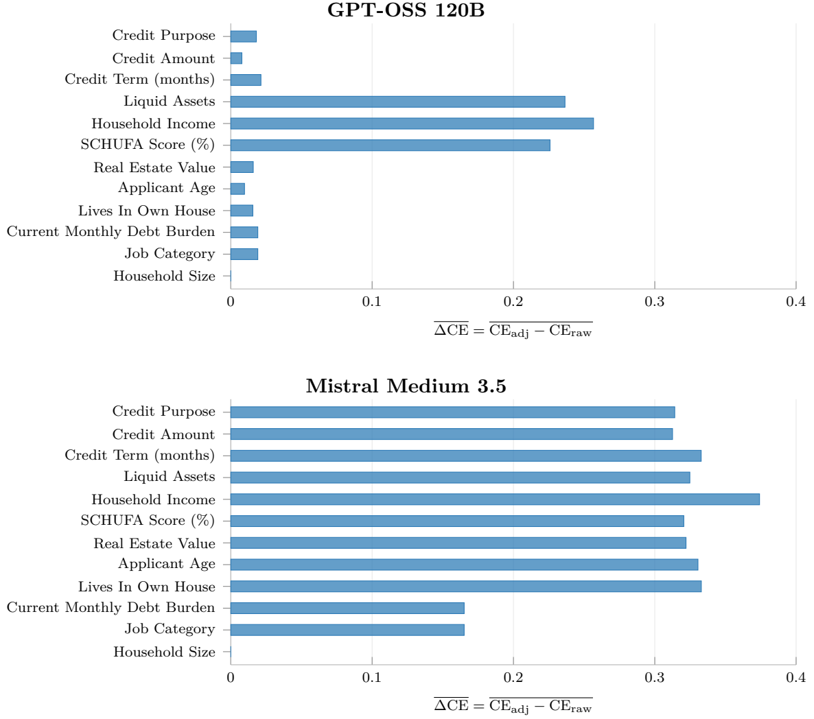
Figure D.8: Mean normalization adjustment for each New German Credit concept, averaged across the 30 questions.
