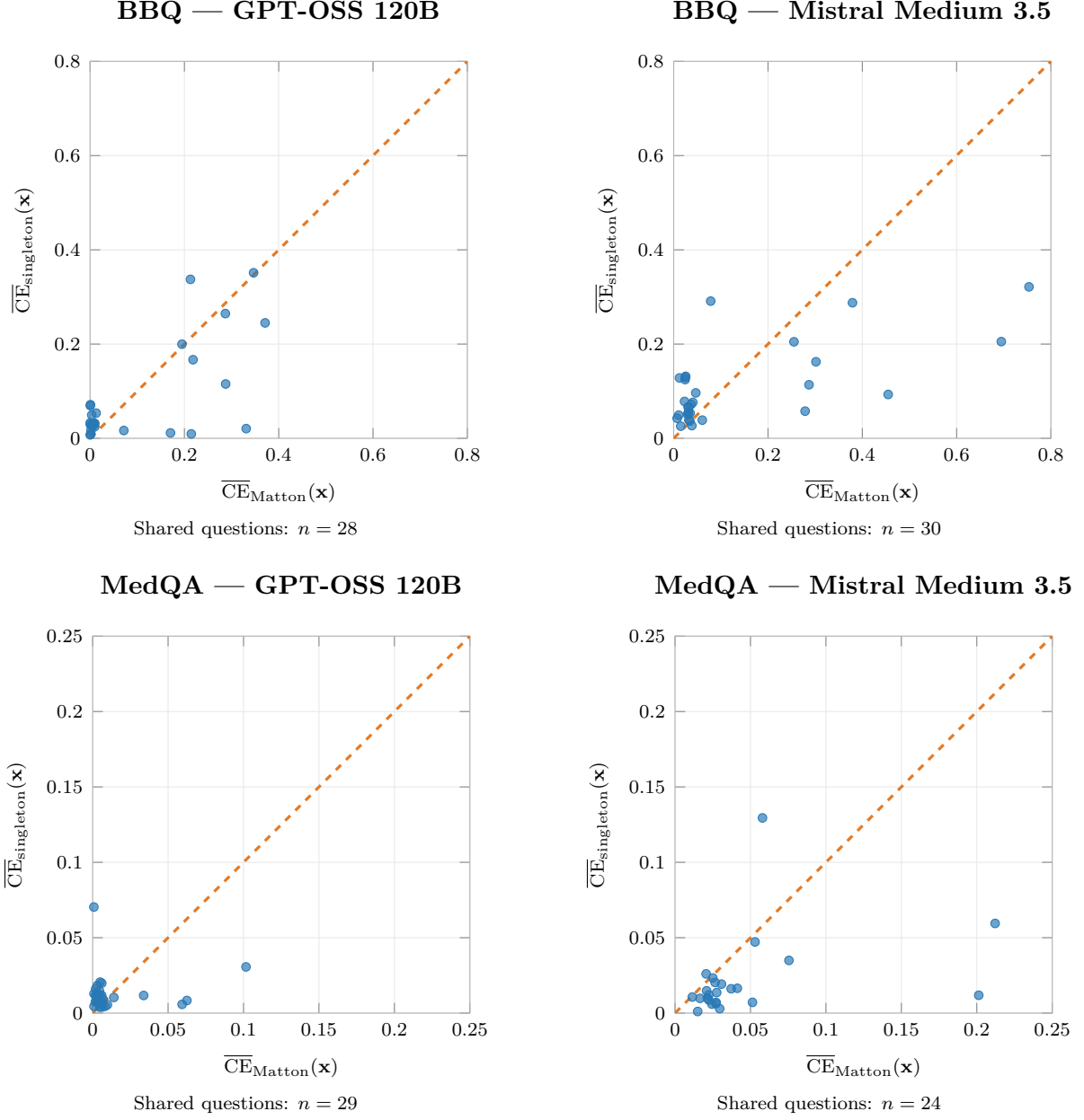
Figure D.4: Question-averaged causal effects produced by FELICS with n_{\max} = 1 and the original Matton implementation for the natural-language comparisons.
