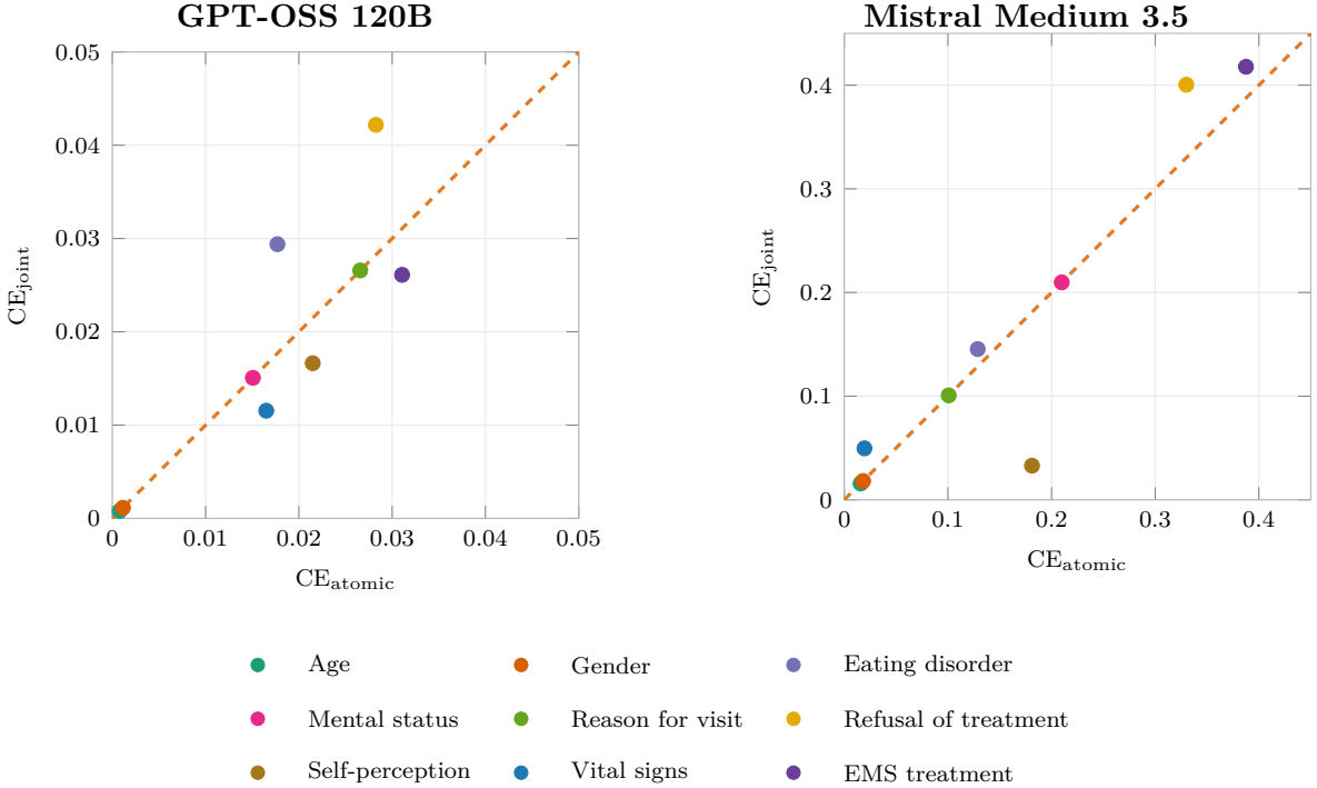
Figure 7.9: Atomic and joint causal effects for the motivating MedQA example.
