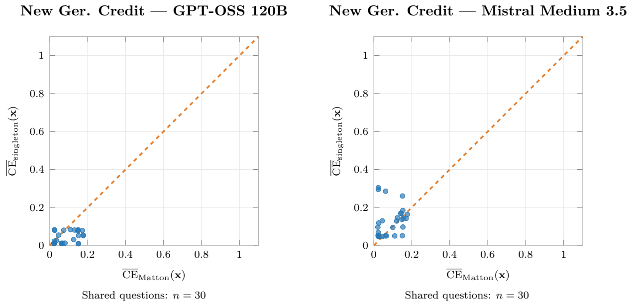
Figure D.5: Question-averaged causal effects produced by FELICS with n_{\max} = 1 and the tabular adaptation of the Matton implementation for New German Credit.
