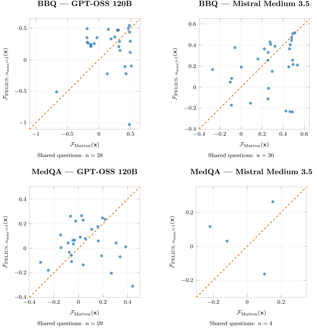
Figure 7.6: Question-level faithfulness produced by FELICS with n_{\max} = 1 and the original Matton implementation for the four completed natural-language comparisons. The dashed orange line denotes exact identity.
