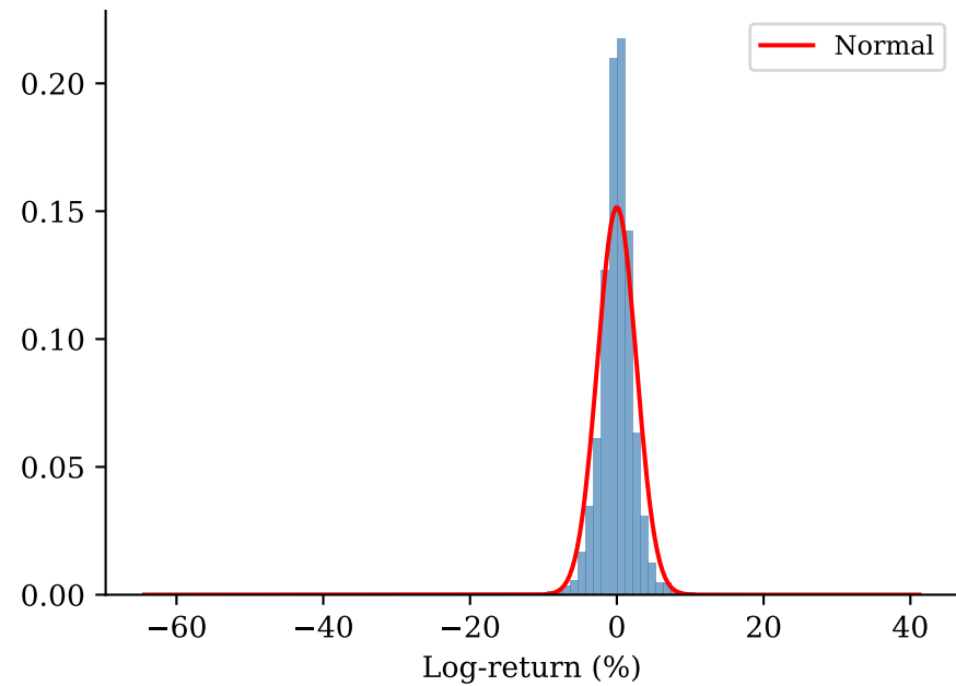
Oil
