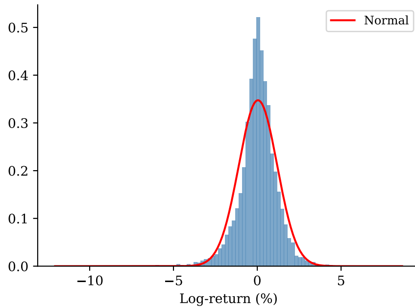
Gold
