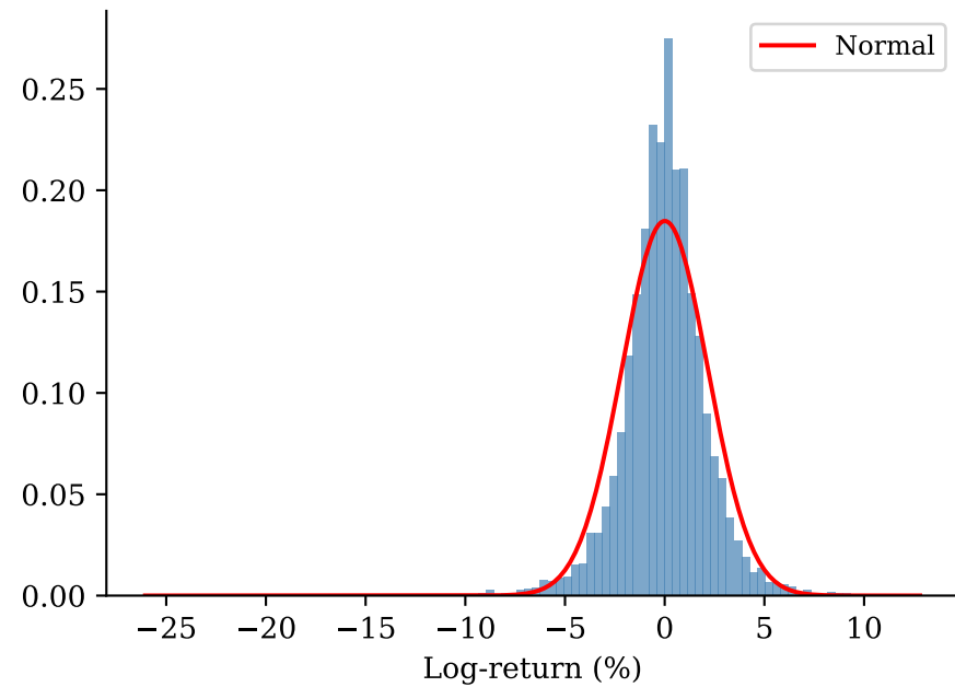
Cocoa
