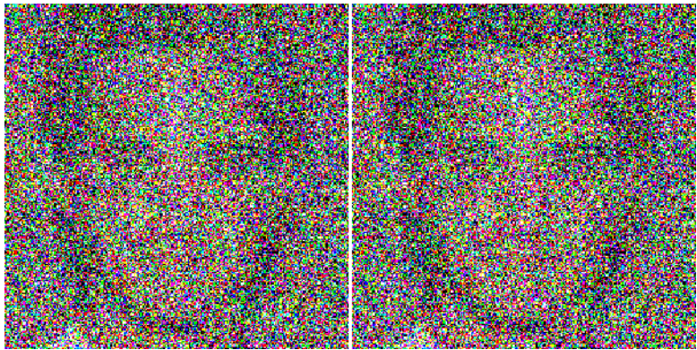
control 1, Tweedie-denoised
