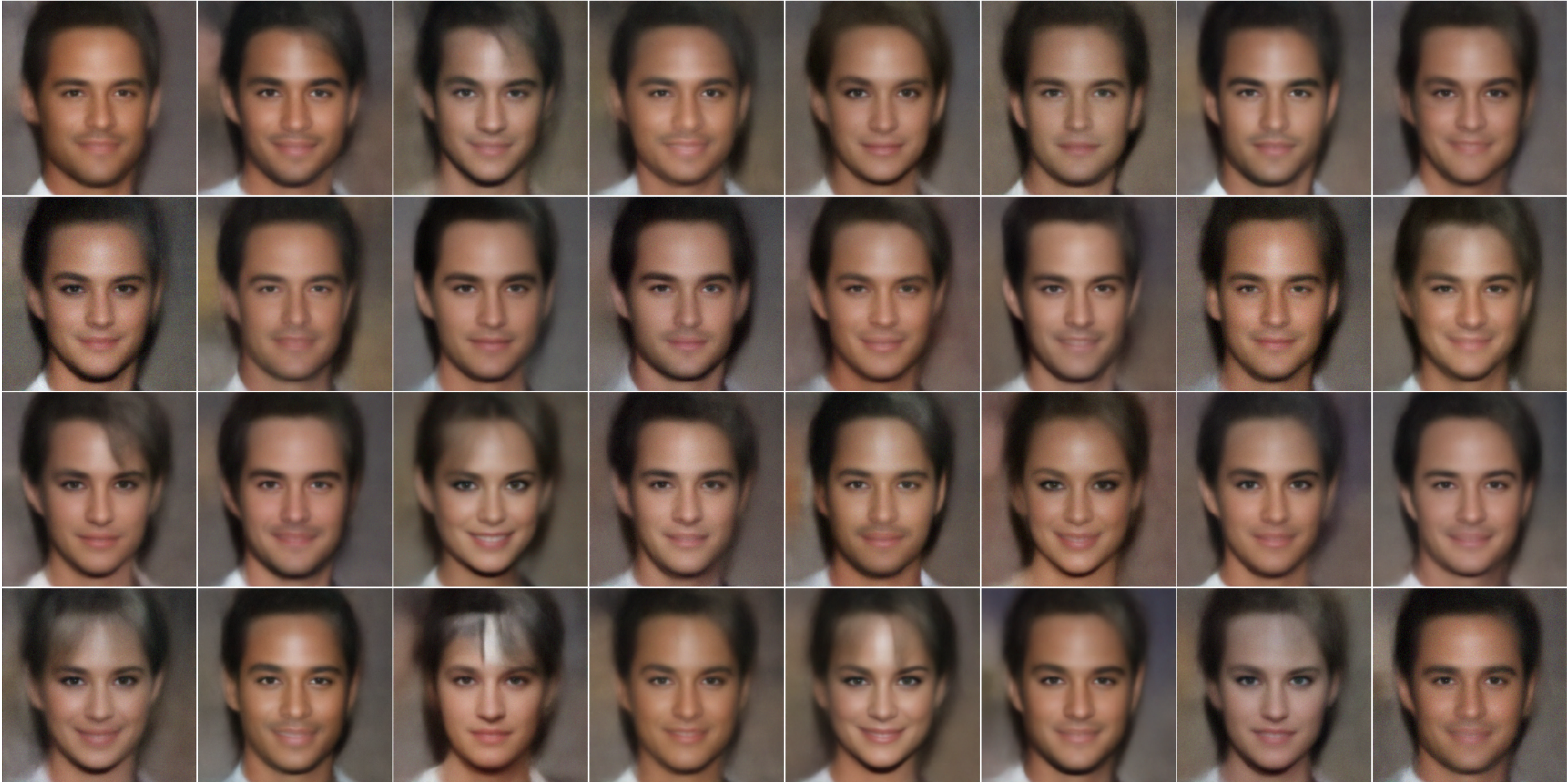
control 2, Tweedie-denoised
