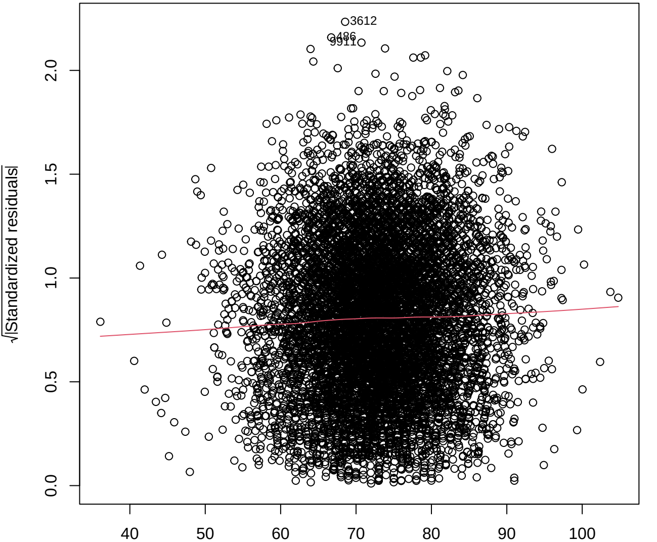
Scale-Location
