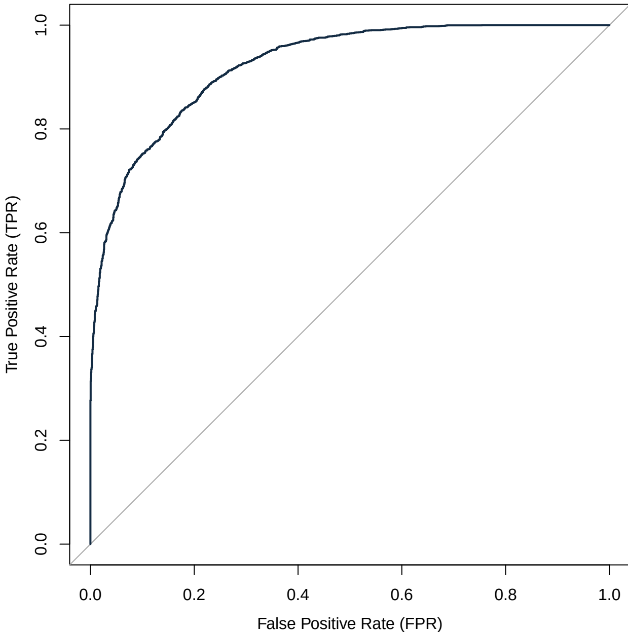
XGBoost ROC Curve (AUC = 0.9235)
