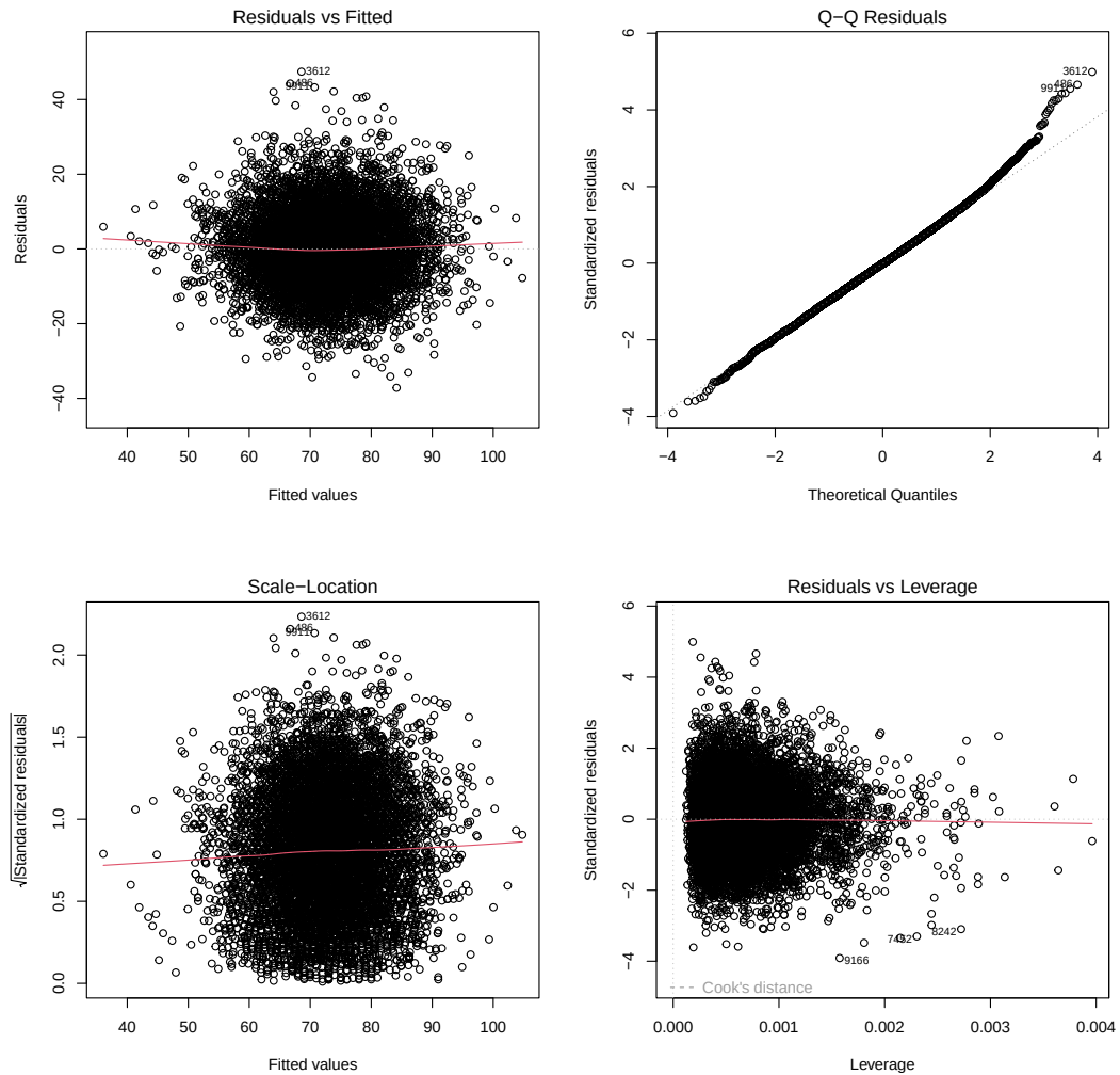
Figure 9. Diagnostic Plots for the Men's Linear Regression Model
