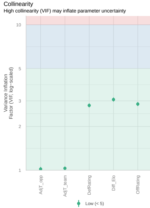
Figure 12. VIF Plot for the Women's Linear Regression Model
