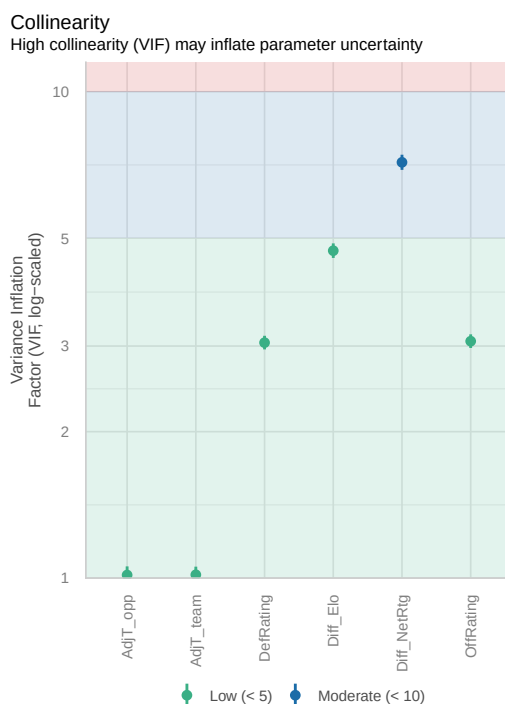
Figure 11. VIF Plot for the Men's Linear Regression Model
