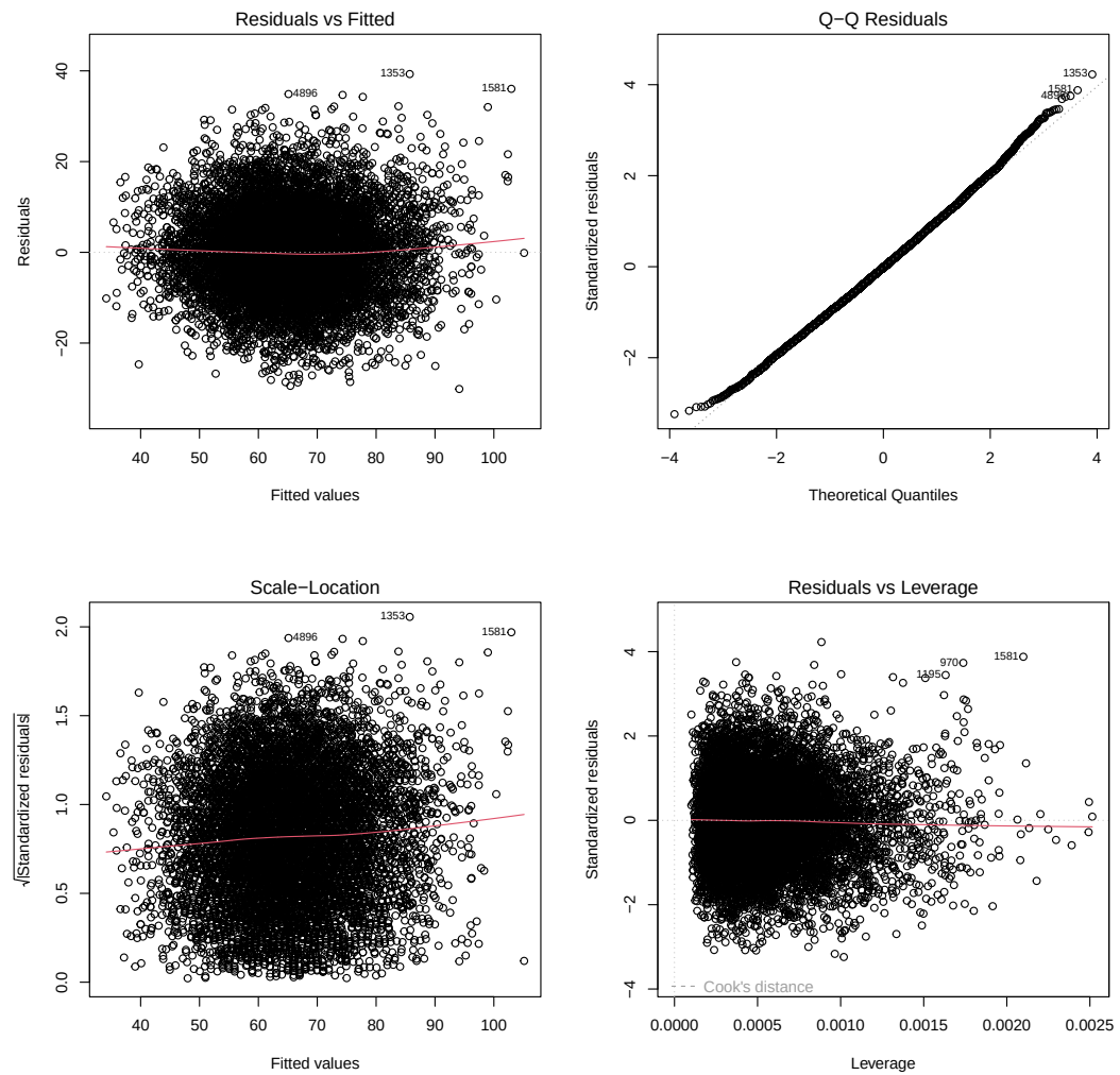
Figure 10. Diagnostic Plots for the Women's Linear Regression Model
