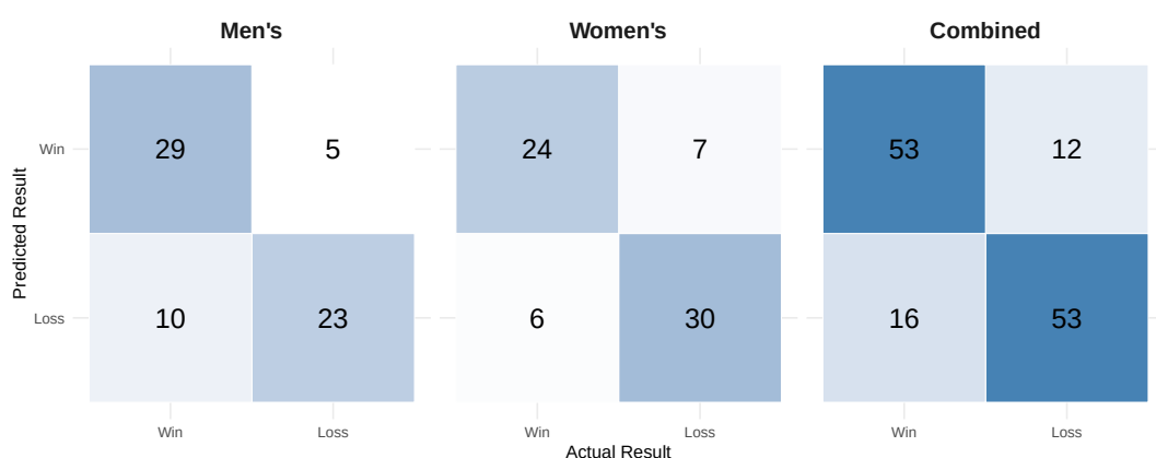
Figure 9. Confusion Matrices for the 2025 XGBoost Model
