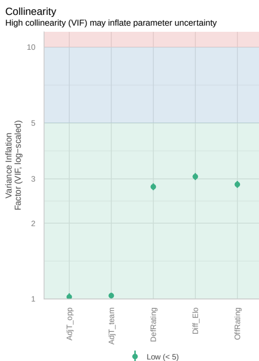
Figure 13. VIF Plot for the Women's Linear Regression Model
