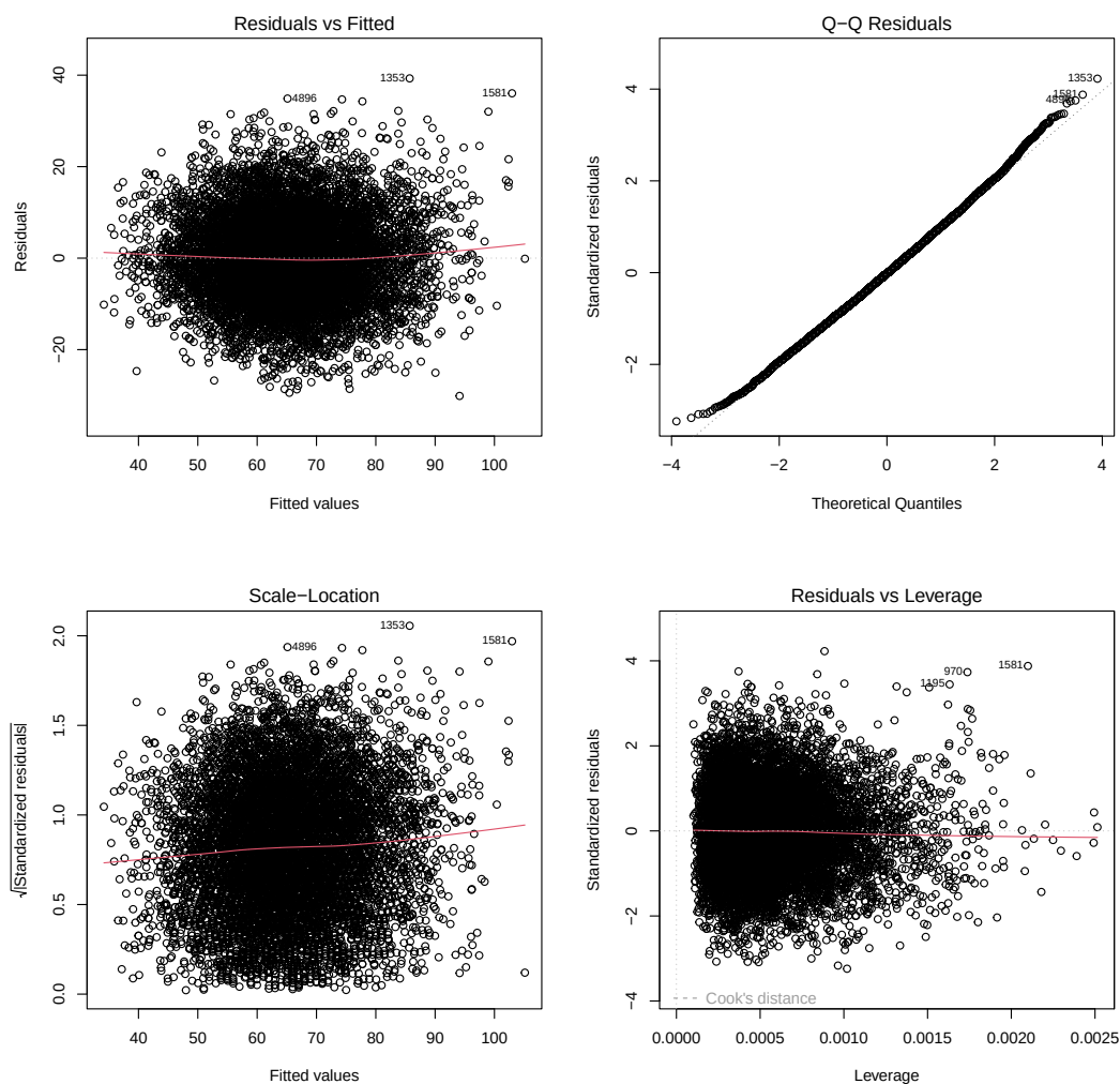
Figure 11. Diagnostic Plots for the Women's Linear Regression Model
