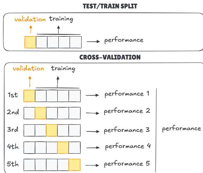
Figure 7. Example of Cross Validation and Regular Test/Train Split [24]
