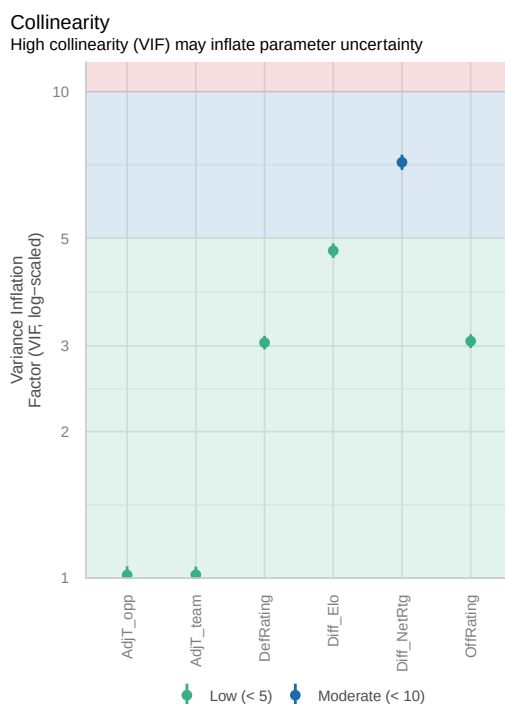
Figure 12. VIF Plot for the Men’s Linear Regression Model
