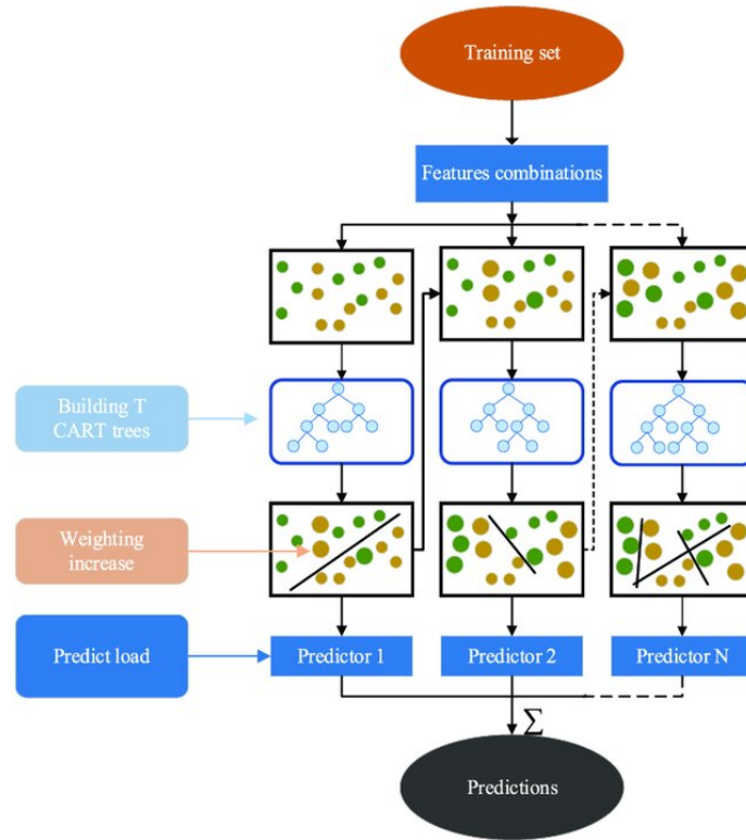
Figure 3. An XGBoost Example [36]
