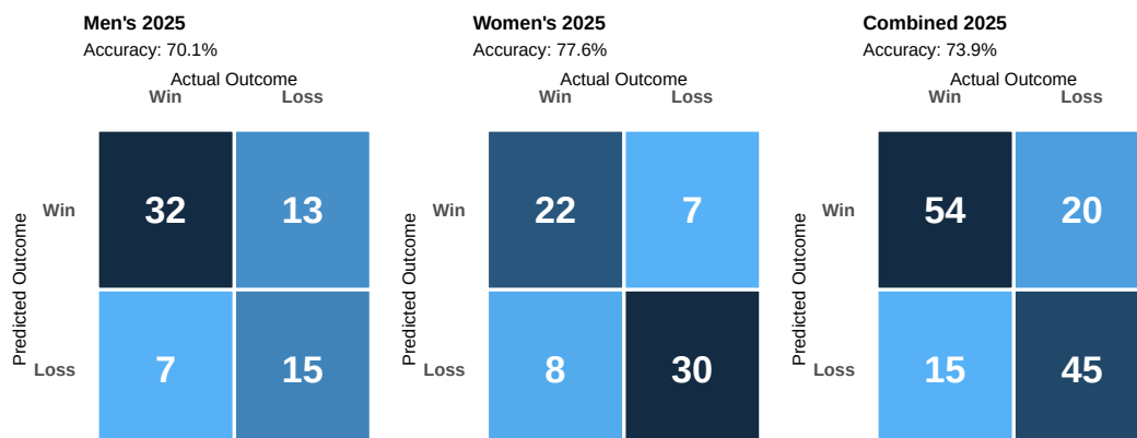
Figure 4. Confusion Matrices for the 2025 Logistic Regression Models
