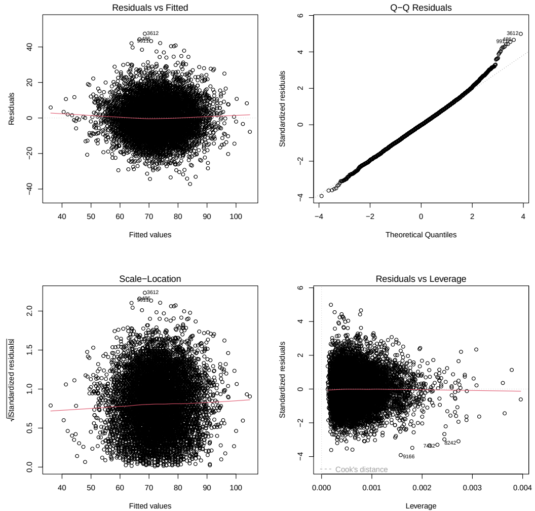
Figure 10. Diagnostic Plots for the Men's Linear Regression Model
