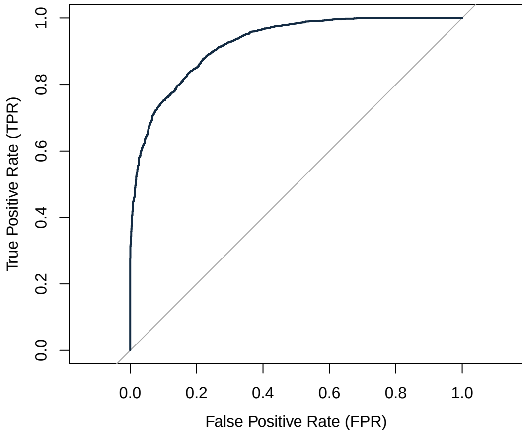
XGBoost ROC Curve (AUC = 0.9235)
