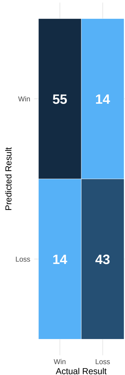
Base – Combined
