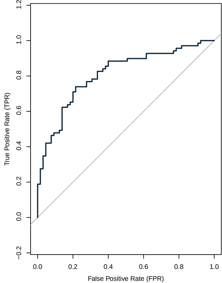
Logistic Regression (AUC = 0.8098)
