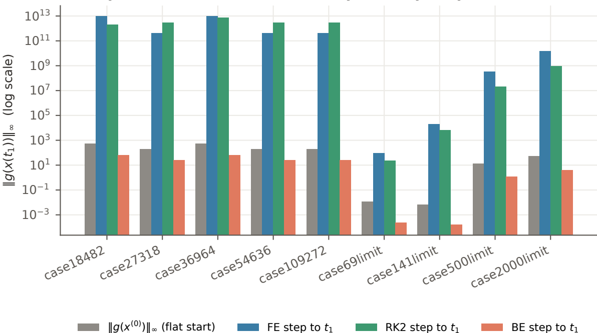
One step to t_1 = 0.005 with K = 10^{-4} : explicit steps explode, BE contracts
