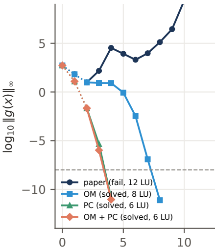
rescue: case36964, S2 ( \Delta t_0 = 0.05 , K = 10^{-3} )
