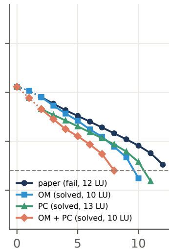
speed-up: case14limit, S1 ( \Delta t_0 = 0.005 , K = 10^{-4} )
