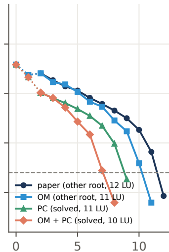
root fixed: case3012wplimit, S1 ( \Delta t_0 = 0.005 , K = 10^{-4} )
