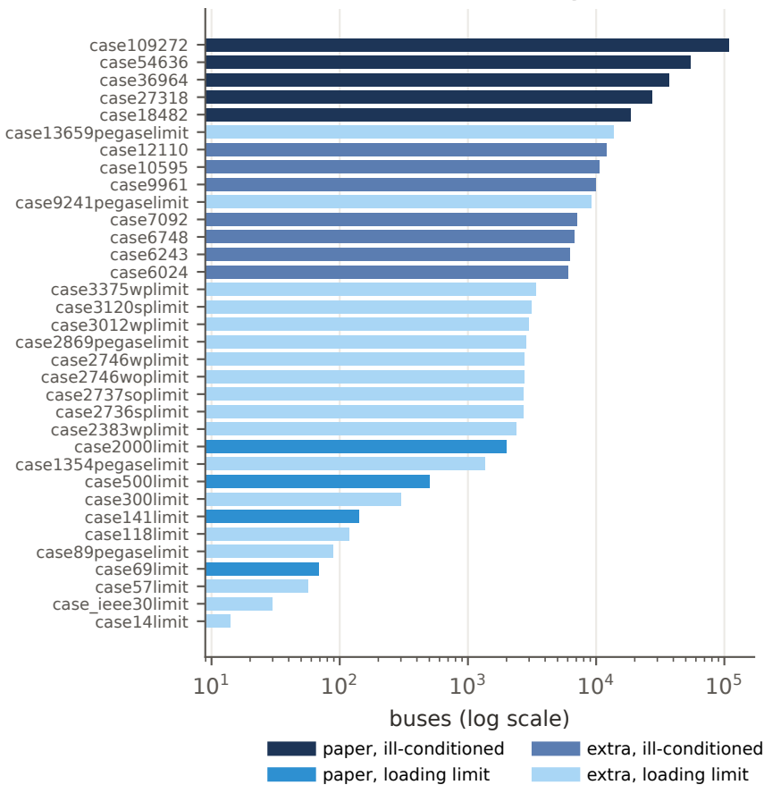
Size of the 34 test systems
