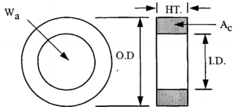
Toroidal Ferrite Core
