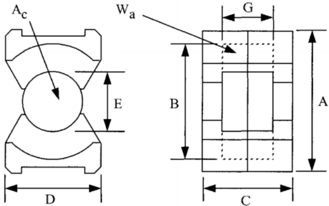
PQ Ferrite Core
