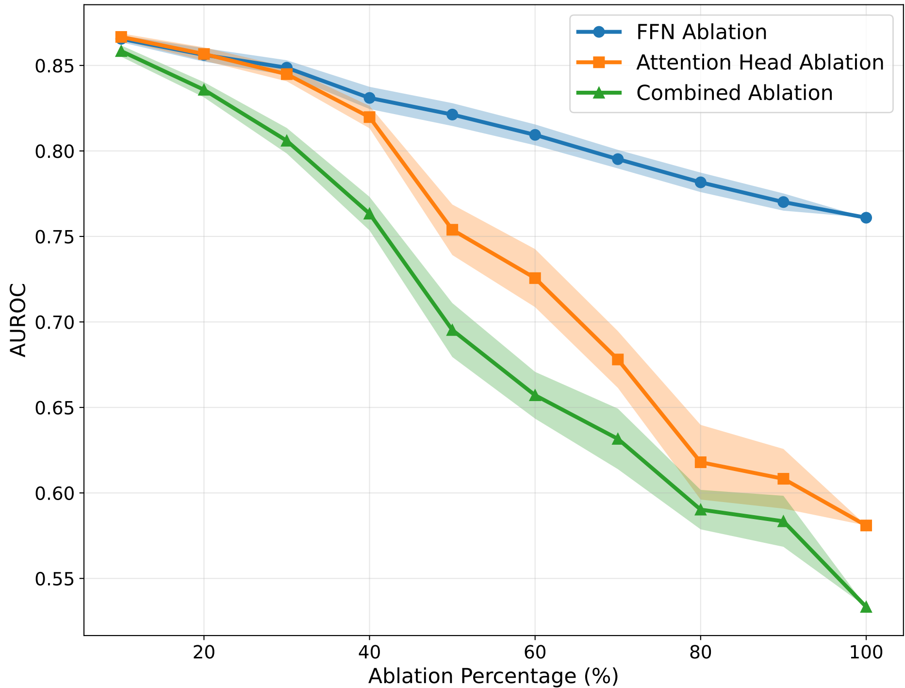
Ablation on LoRA fine-tuned model
