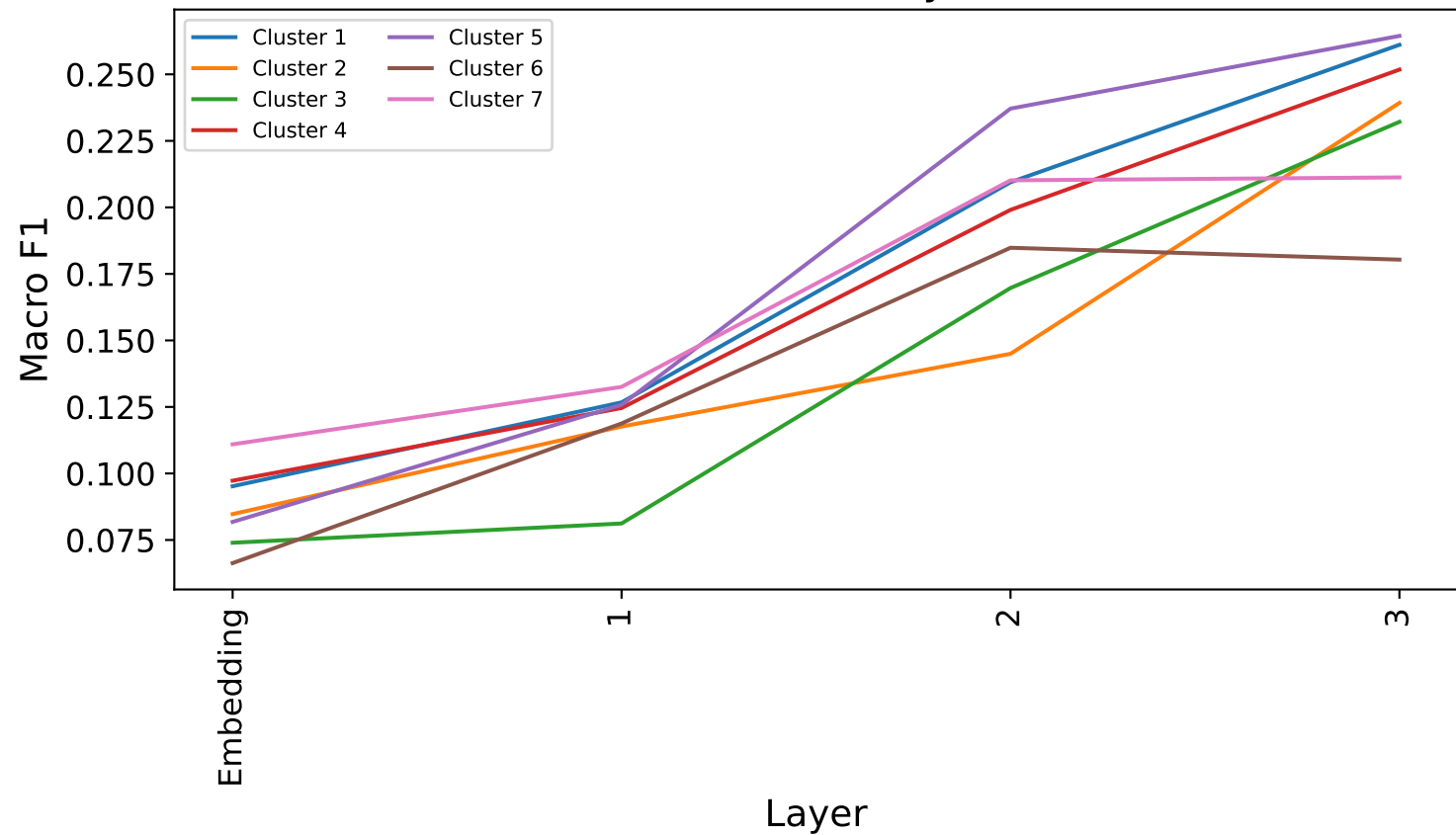
Per-cluster Macro F1 across layers (Frozen Model)
