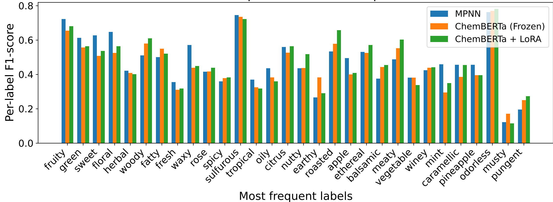
Per-label F1 Comparison of Most Frequent Labels
