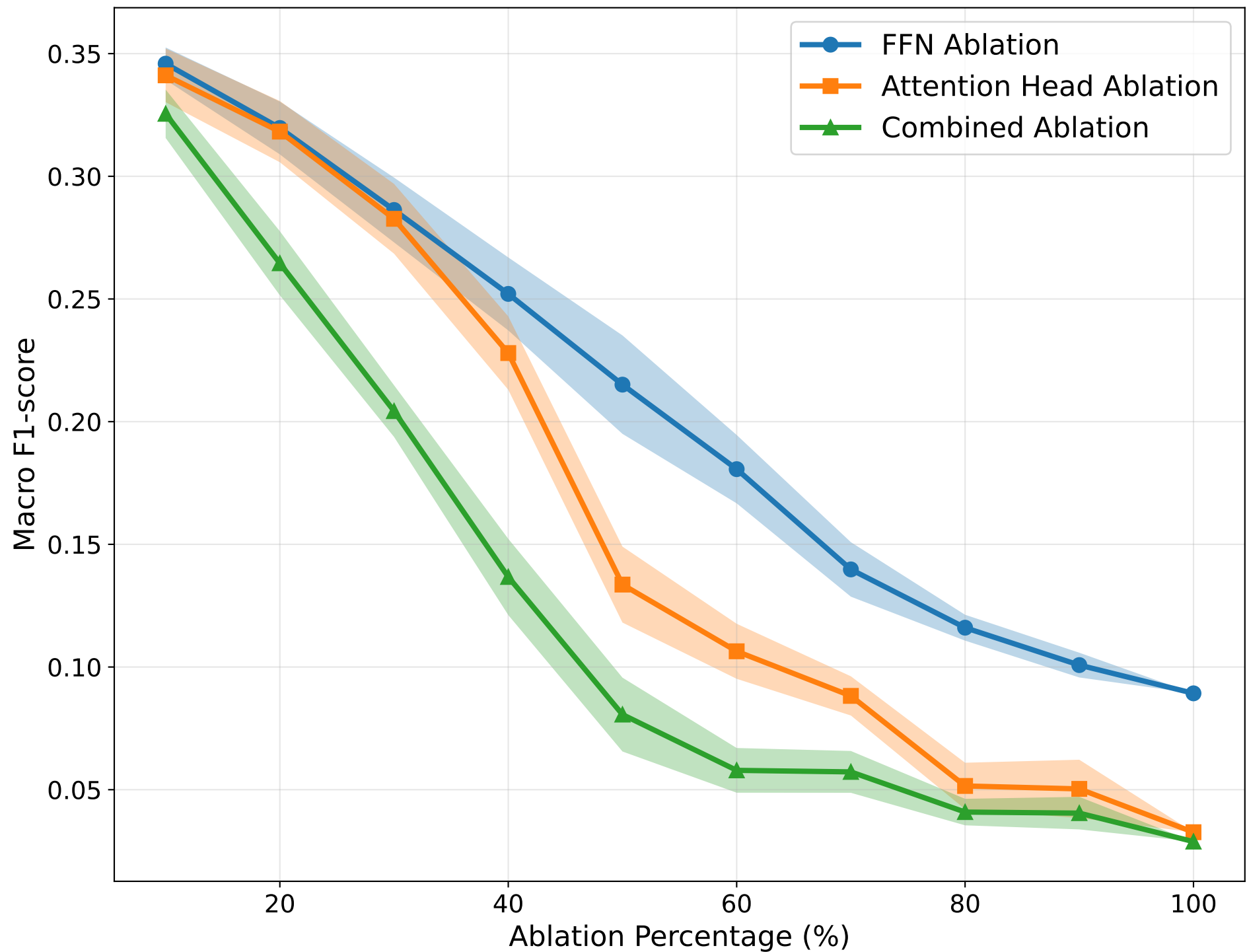
Ablation on LoRA model
