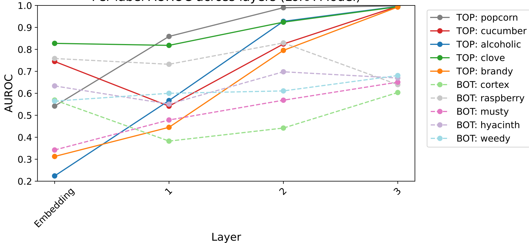
Per-label AUROC across layers (LoRA Model)
