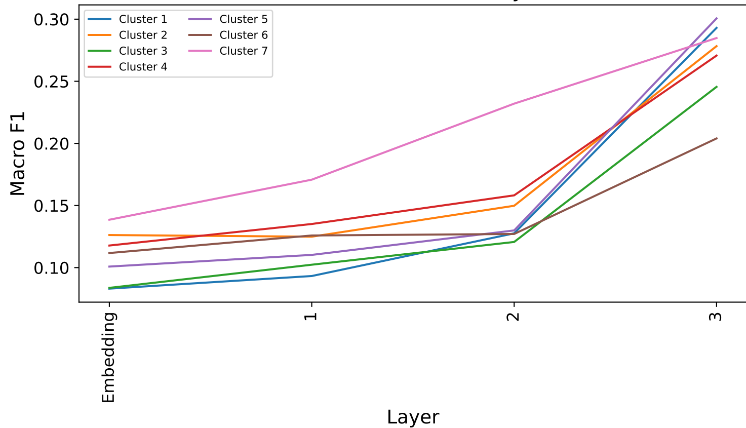
Per-cluster Macro F1 across layers (LoRA)
