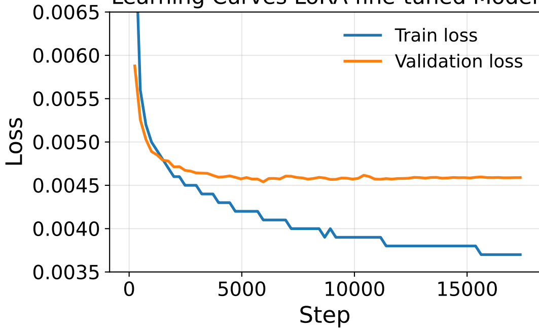
Learning Curves LoRA fine-tuned Model
