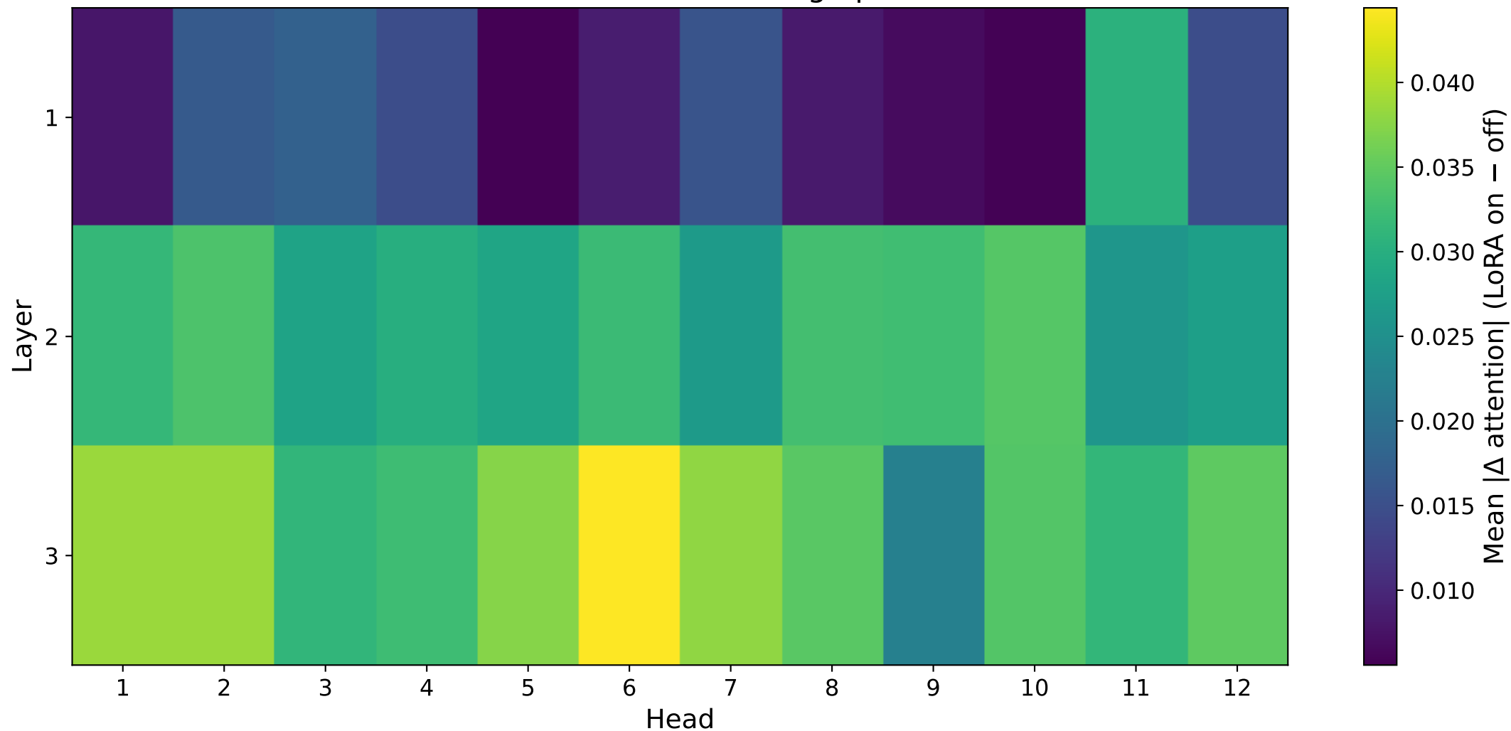
LoRA-induced attention change per head
