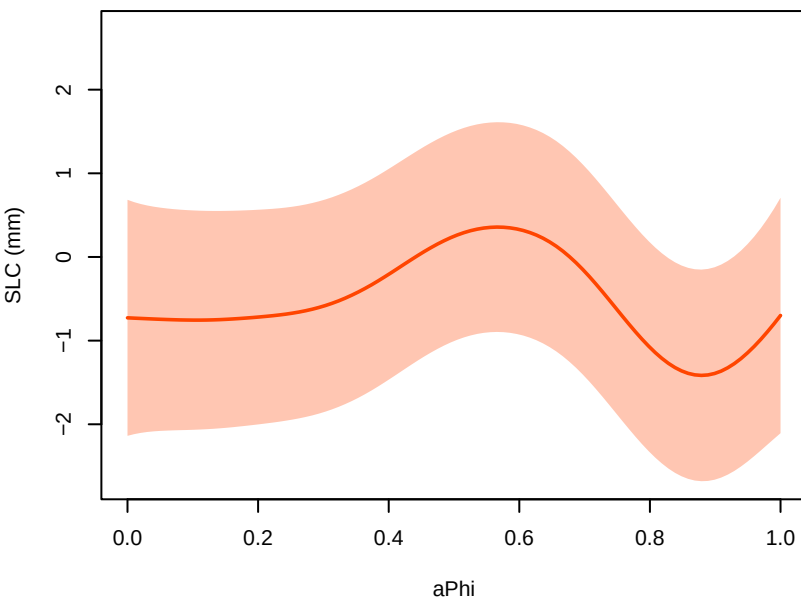
smb+thermal_forcing – parameter main effects at 2021 (other params at 0.5; forcing at EC–Earth3–Veg, ssp585)
