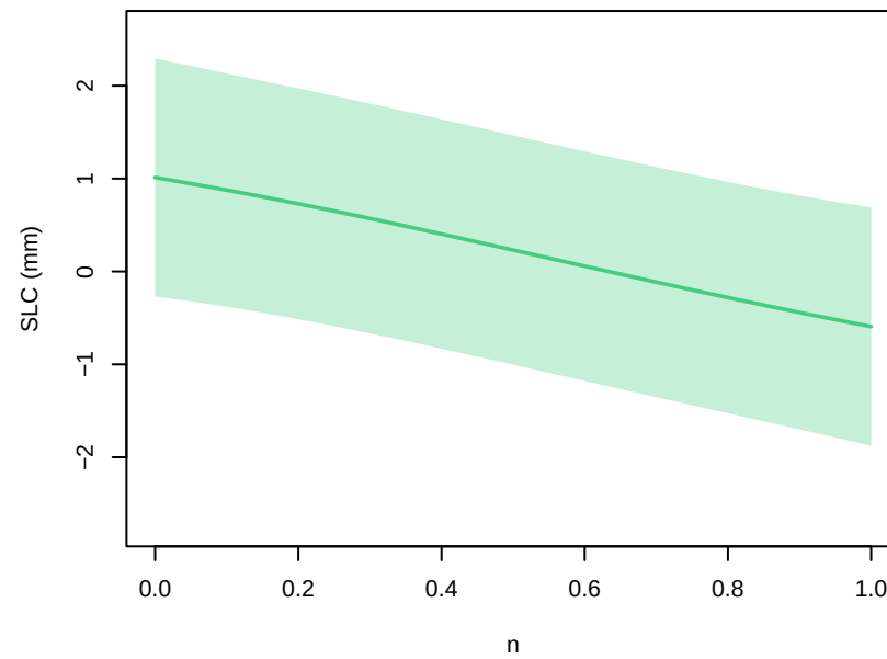
GMSTa+thermal_forcing – parameter main effects at 2021 (other params at 0.5; forcing at EC–Earth3–Veg, ssp585)
