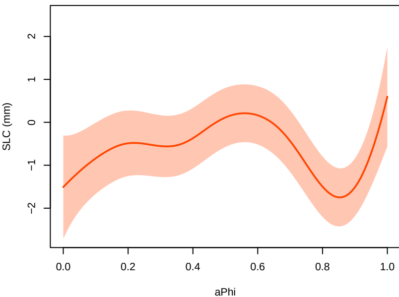
GMSTa+thetao – parameter main effects at 2021 (other params at 0.5; forcing at EC-Earth3-Veg, ssp585)
