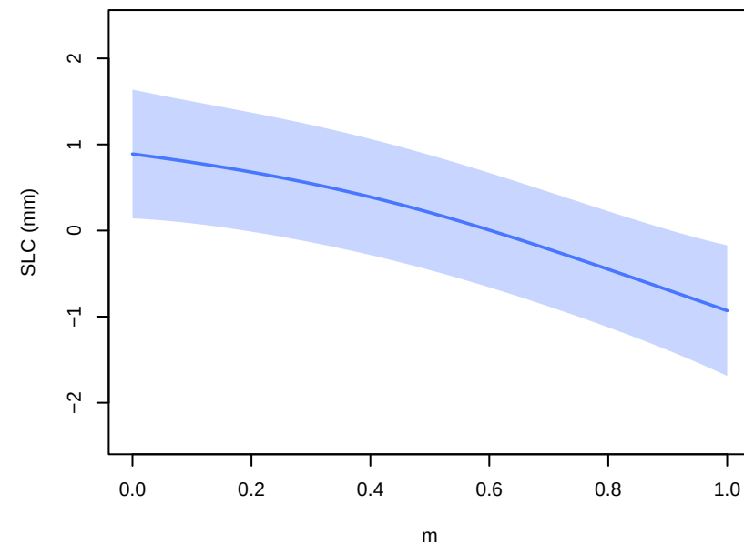
tas+thetao – parameter main effects at 2021 (other params at 0.5; forcing at EC–Earth3–Veg, ssp585)
