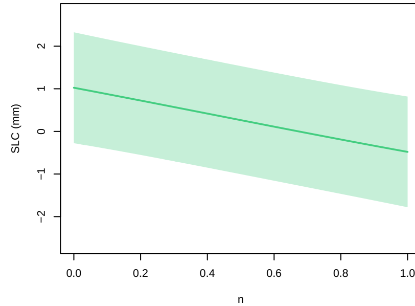
tas – parameter main effects at 2021 (other params at 0.5; forcing at EC–Earth3–Veg, ssp585)
