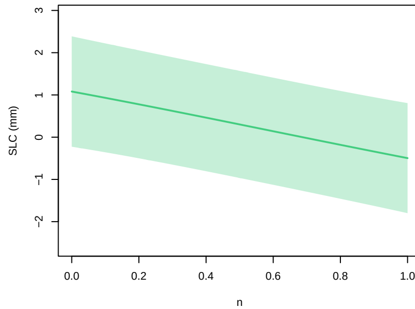
thermal_forcing – parameter main effects at 2021 (other params at 0.5; forcing at EC–Earth3–Veg, ssp585)
