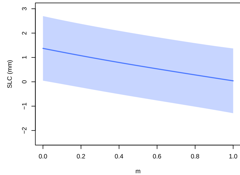
smb – parameter main effects at 2021 (other params at 0.5; forcing at EC–Earth3–Veg, ssp585)
