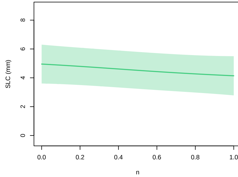
GMSTa+thermal_forcing – parameter main effects at 2021 (other params at 0.5; forcing at MIROC-ES2L, ssp585)
