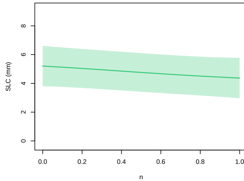
smb – parameter main effects at 2021 (other params at 0.5; forcing at MIROC-ES2L, ssp585)
