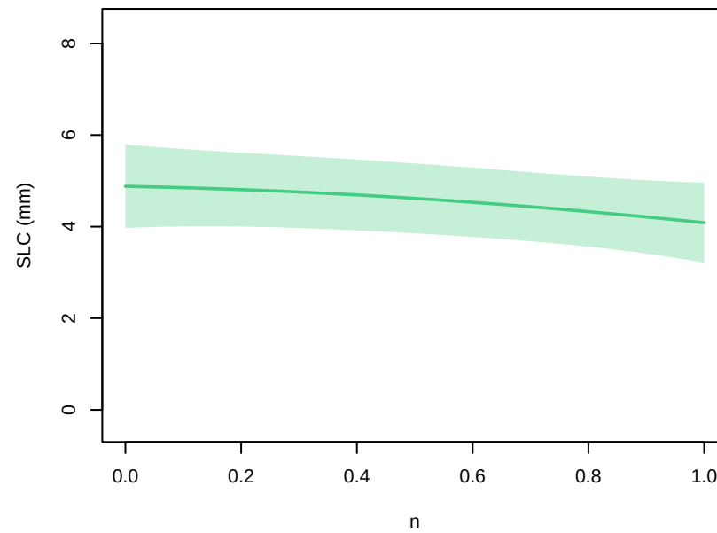
tas+thetao – parameter main effects at 2021 (other params at 0.5; forcing at MIROC-ES2L, ssp585)
