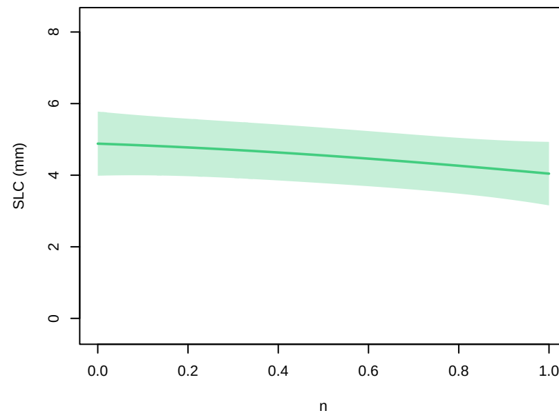
thetao – parameter main effects at 2021 (other params at 0.5; forcing at MIROC-ES2L, ssp585)
