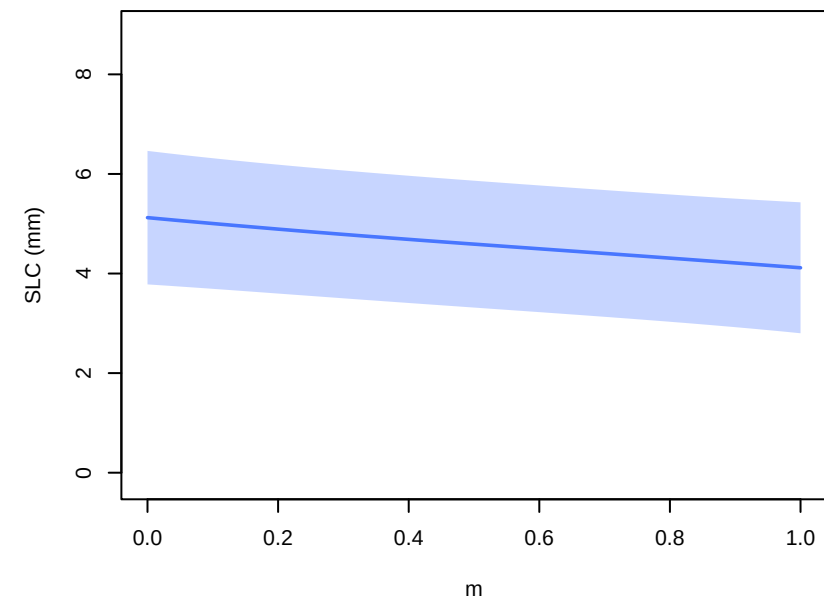
smb+thermal_forcing – parameter main effects at 2021 (other params at 0.5; forcing at MIROC-ES2L, ssp585)
