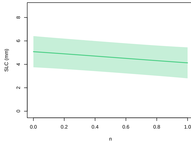
thermal_forcing – parameter main effects at 2021 (other params at 0.5; forcing at MIROC-ES2L, ssp585)
