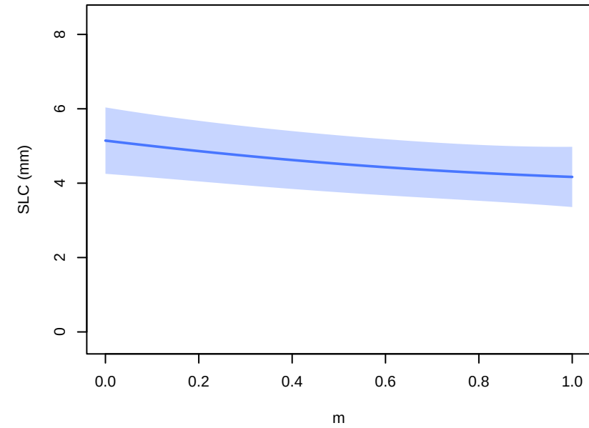
GMSTa+thetao – parameter main effects at 2021 (other params at 0.5; forcing at MIROC-ES2L, ssp585)
