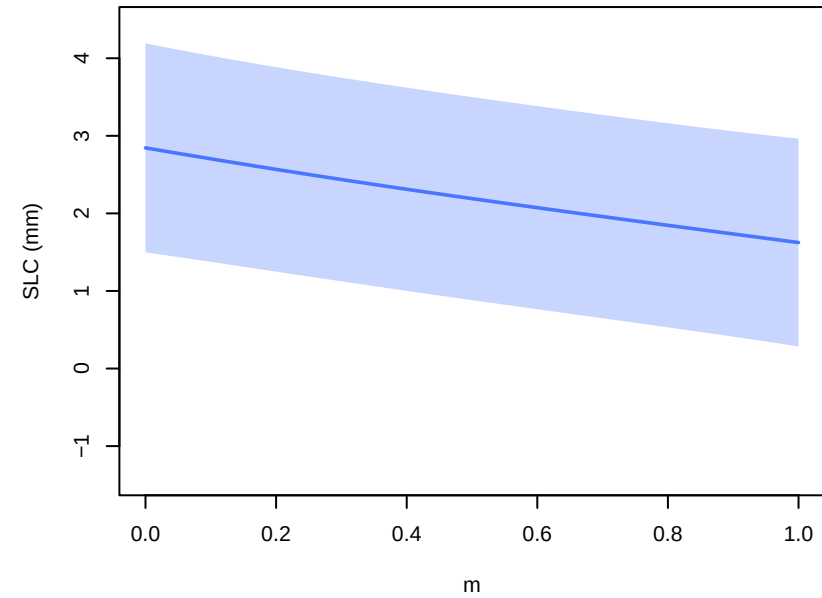
smb – parameter main effects at 2021 (other params at 0.5; forcing at MRI-ESM2-0, ssp585)
