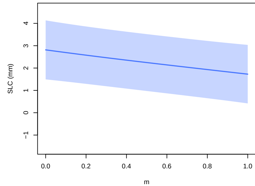
thermal_forcing – parameter main effects at 2021 (other params at 0.5; forcing at MRI-ESM2-0, ssp585)
