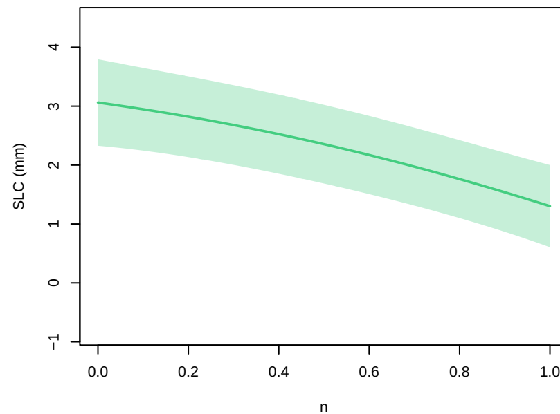
tas+thetao – parameter main effects at 2021 (other params at 0.5; forcing at MRI-ESM2-0, ssp585)
