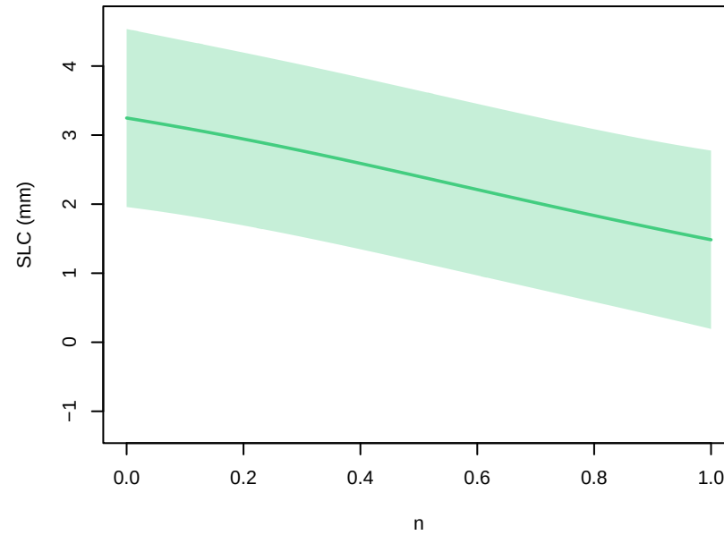
GMSTa+thermal_forcing – parameter main effects at 2021 (other params at 0.5; forcing at MRI-ESM2-0, ssp585)
