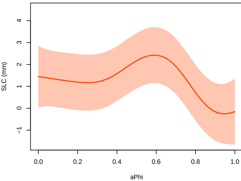
smb+thermal_forcing – parameter main effects at 2021 (other params at 0.5; forcing at MRI-ESM2-0, ssp585)
