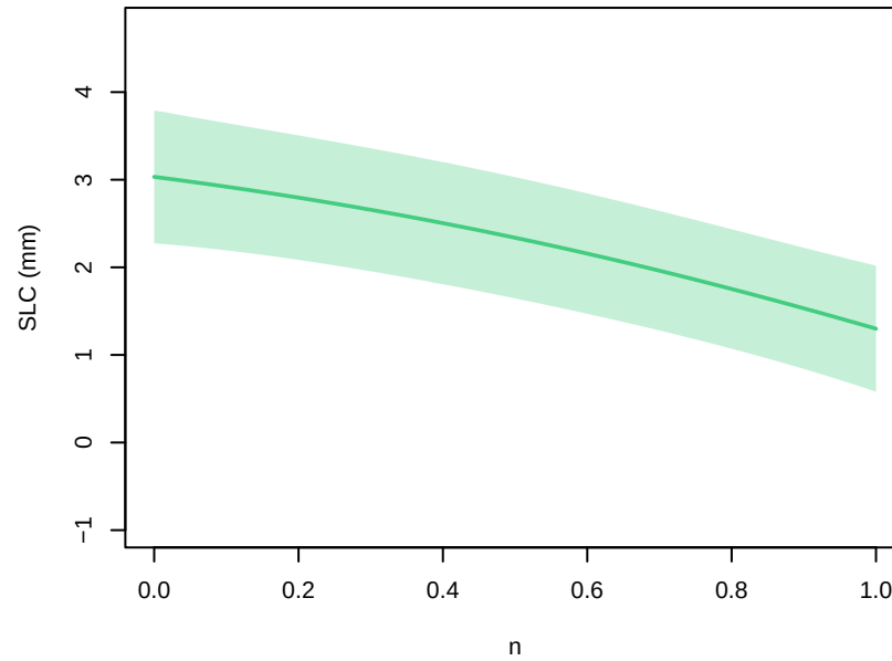
GMSTa+thetao – parameter main effects at 2021 (other params at 0.5; forcing at MRI-ESM2-0, ssp585)
