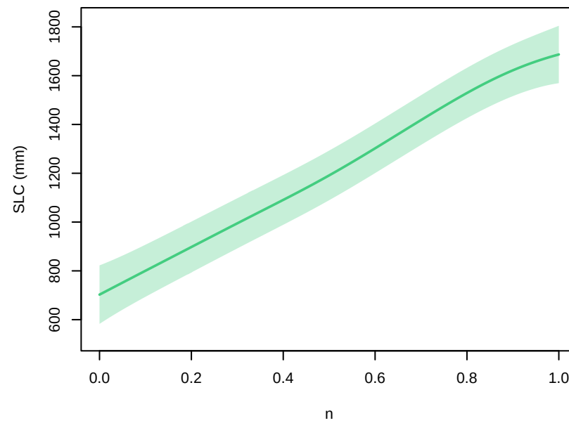
thermal_forcing – parameter main effects at 2300 (other params at 0.5; forcing at CESM2-WACCM, ssp585)
