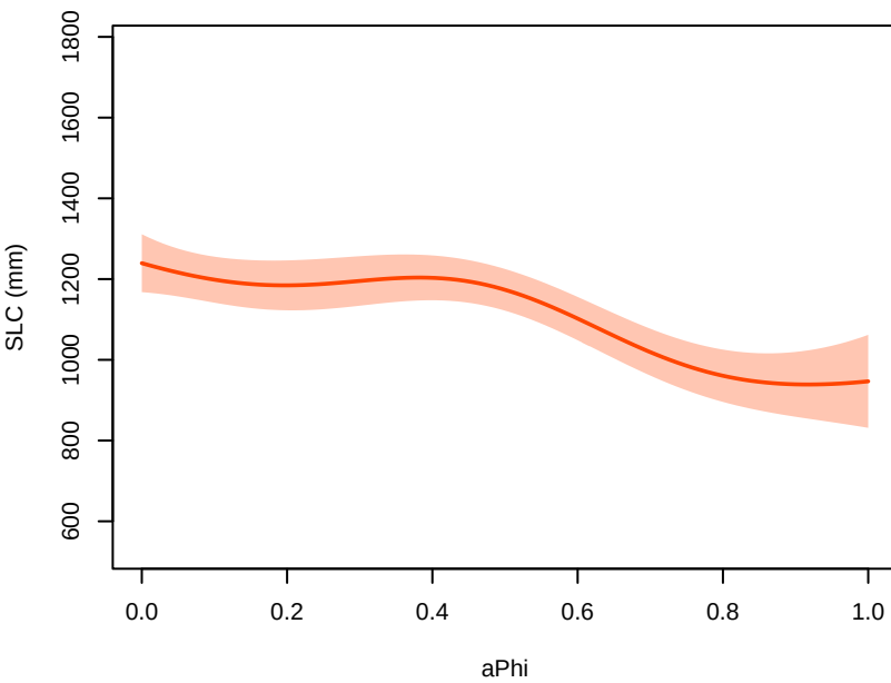
GMSTa+thetao – parameter main effects at 2300 (other params at 0.5; forcing at CESM2–WACCM, ssp585)
