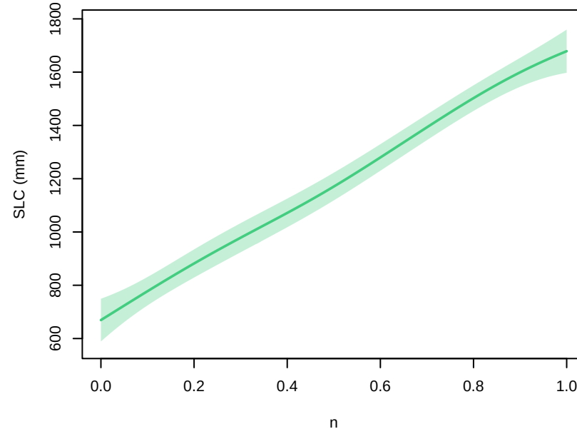
GMSTa+thermal_forcing – parameter main effects at 2300 (other params at 0.5; forcing at CESM2–WACCM, ssp585)
