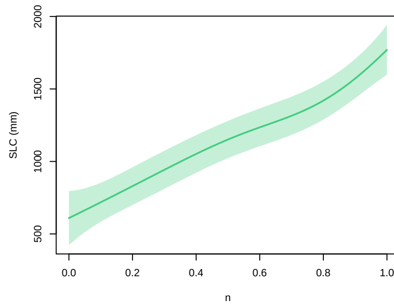
smb – parameter main effects at 2300 (other params at 0.5; forcing at CESM2–WACCM, ssp585)
