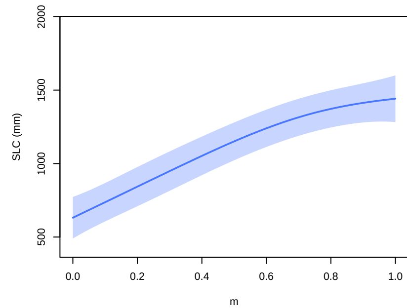
smb – parameter main effects at 2300 (other params at 0.5; forcing at CESM2–WACCM, ssp585)
