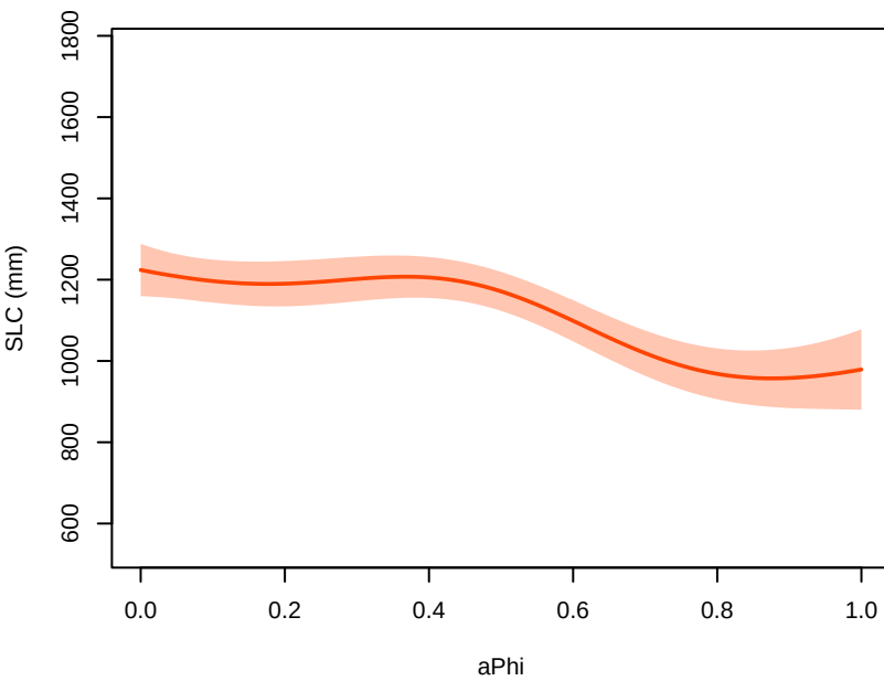
tas+thetao – parameter main effects at 2300 (other params at 0.5; forcing at CESM2–WACCM, ssp585)
