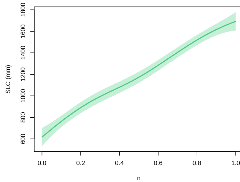
GMSTa+thetao – parameter main effects at 2300 (other params at 0.5; forcing at CESM2–WACCM, ssp585)
