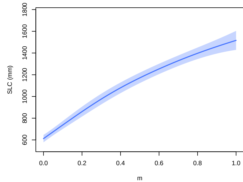
tas+thetao – parameter main effects at 2300 (other params at 0.5; forcing at CESM2–WACCM, ssp585)
